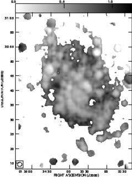
Fig. 9. Total spectral index map of M33 as determined between the two wavelengths 3.6 and 20 cm. The angular resolution is 90'' . For the total intensity maps, 3\sigma level was considered to obtain this spectral index map.
