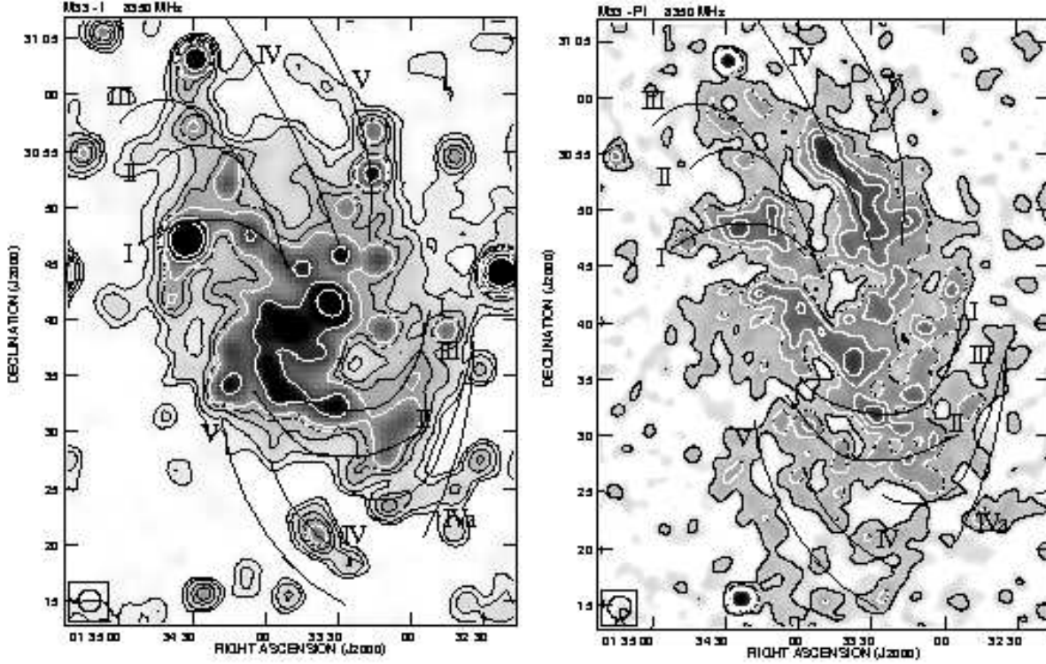
Fig. 3. A sketch of the optical arms (Sandage & Humphreys 1980) overlaid on the total (left panel) and linearly polarized (right panel) intensities at 3.6 cm. Grey scales and Contour levels are the same as in Figs. 1 and 2.
