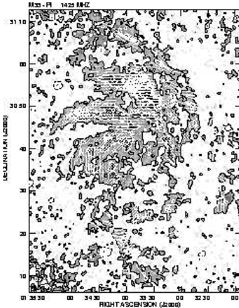
Fig. 8. The combined VLA + Effelsberg map of the linearly polarized emission (contours and grey scale) and degree of polarization (vector lengths) from M33 at 20 cm. The HPBW is 51'' (the beam area is shown in the left-hand corner). Contour levels are 0.07, 0.14, 0.21, 0.28, 0.42, 0.56, 0.84 mJy/beam. The rms noise is 0.015 mJy/beam. A vector length of 51'' represents a degree of polarization of 8.7%.
