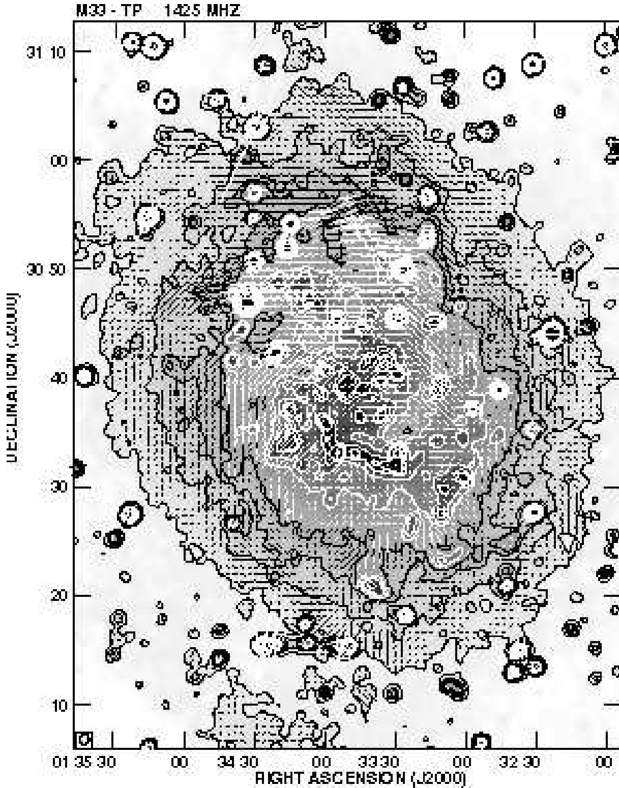
Fig. 7. The combined VLA + Effelsberg map of the total intensity emission from M33 at 20 cm, with apparent B-vectors of polarized intensity (E-vectors rotated by 90^\circ ) superimposed. The HPBW is 51'' (the beam area is shown in the left-hand corner). Contour levels are 0.3, 0.6, 0.9, 1.2, 1.8, 2.4, 3.6, 4.8, 9.6, 19.2 mJy/beam. The rms noise is 0.07 mJy/beam in total intensity and 0.025 mJy/beam in polarization. The vectors were plotted starting from 1.5\sigma . A vector length of 51'' represents a polarized intensity of 0.1 mJy/beam.
