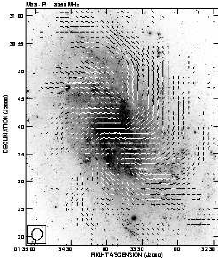
Fig. 4. Apparent B-vectors (E-vectors rotated by 90^\circ ) at 3.6 cm superimposed on an optical image (B-band, taken from the STScI Digitized Sky Survey) of M33. A vector length of 1' represents a polarized intensity of 0.3 \text{ mJy/beam} . The vectors were plotted starting from 1.5\sigma .
