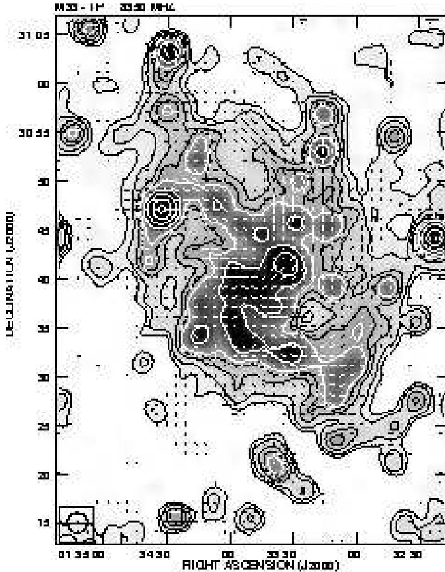
Fig. 1. Total intensity emission from M33 at 3.6 cm observed with the Effelsberg telescope, with apparent B-vectors (E-vectors rotated by 90^\circ ) of polarized intensity superimposed. The HPBW is 120'' (the beam area is shown in the left-hand corner). Contour levels are 0.5, 1, 2, 3, 4, 8, 16, 32, 64 mJy/beam. The rms noise is 0.14 mJy/beam in total intensity and 0.04 mJy/beam in linear polarization. The vectors were plotted starting from 0.1 mJy/beam ( 2.5\sigma ). A vector length of 1' represents a polarized intensity of 0.5 mJy/beam.
