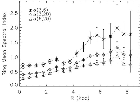
Fig. 11. Total spectral index averaged in rings of 0.5 kpc width in the galactic plane versus the radial distance from the center of M33. For the total intensity maps, one \sigma level was considered before integration.
