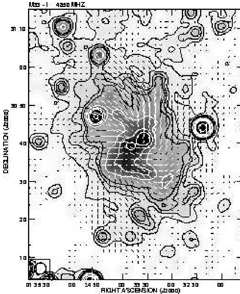
Fig. 5. Total intensity emission from M33 at 6.2 cm observed with the Effelsberg telescope, with an angular resolution of 180'' (the beam area is shown in the left-hand corner). Apparent B-vectors of the polarized intensity (E-vectors rotated by 90^\circ ) are superimposed. Contour levels are 2.2, 4.4, 6.6, 8.8, 17.6, 26.4, 35.2, 70.4 mJy/beam. The rms noise is 0.56 mJy/beam in total intensity and 0.12 mJy/beam in polarization. The vectors were plotted starting from 2.5\sigma . A vector length of 1.5' represents a polarized intensity of 1 mJy/beam.
