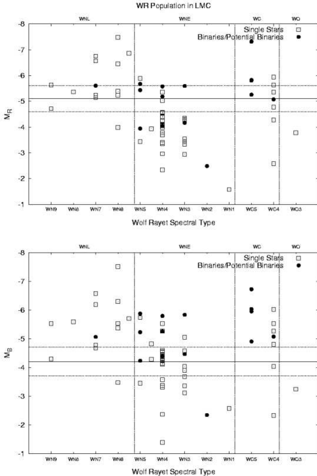
Figure 8. Broadband photometry of W-R stars in the LMC (Massey 2002) compared to the absolute B (bottom) and R (top) magnitude limits. Note that the evolutionary sequence for W-R stars is WN9 \rightarrow WN8 \rightarrow WN7 \rightarrow WN6 \rightarrow WN5 \rightarrow WN4 \rightarrow WN3 \rightarrow WN2 \rightarrow WN1 \rightarrow WC5 \rightarrow WC4 \rightarrow WC3 \rightarrow WO .
