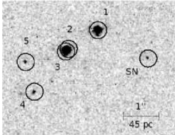
Figure 2. HST image showing SN 2002ap and several neighbouring stellar objects. This image is the sum of the F435W (Aug 2004) and F814W (Jul 2004) HRC observations. Although objects 2 and 3 appear to be a single source in this image, they are detected as two PSFs separated by 3 ACS/HRC pixels ( 0''.075 ) by the PSF-fitting photometry package DOLPHOT. See text for further details.
