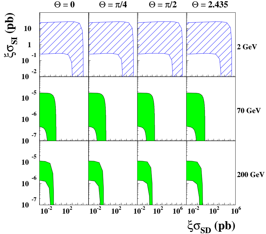
Figure 6: Examples of slices of the 4-dimensional allowed volume ( \xi\sigma_{SI}, \xi\sigma_{SD}, m_W, \theta ) in the considered model frameworks; see text. The hatched slice appears when accounting for the Migdal effect. Analogous remarks as those in the caption of Fig. 4 hold.
