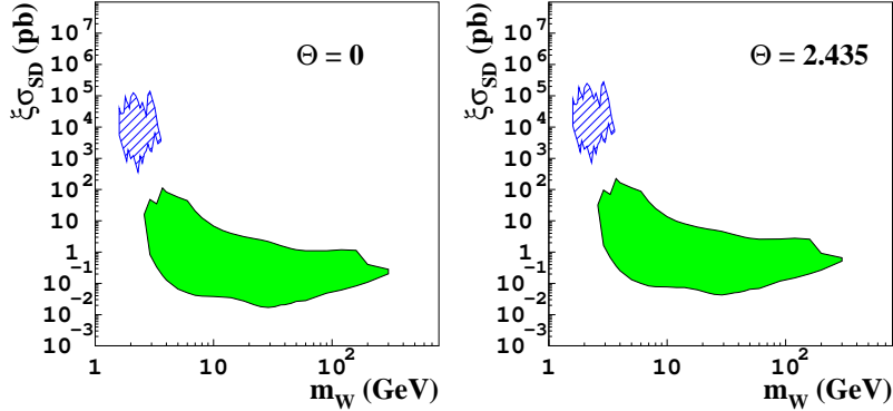
Figure 5: Two slices of the 3-dimensional allowed volume (\xi\sigma_{SD}, m_W, \theta) in the considered model frameworks for pure SD coupling; see text. The hatched regions appear when accounting for the Migdal effect. Analogous remarks as those in the caption of Fig. 4 hold.
