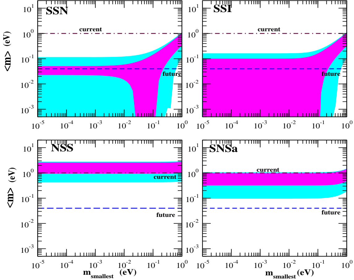
Figure 6: The effective mass \langle m \rangle for scenarios SSN (top left), SSI (top right), NSS (bottom left) and SNSa (bottom right). The magenta shaded (darker) regions correspond to the the best-fit point from Eq. (4) and allowing the phases to take arbitrary values in the interval [0 : 2\pi] . The blue shaded (lighter) regions are obtained by varying the mass and mixing angles as well in the allowed ranges from Eqs. (3) and (6). We assumed that \Delta m_{s1}^2 = \Delta \tilde{m}_{s1}^2 and \Delta m_{s2}^2 = \Delta \tilde{m}_{s2}^2 . Scenario ISS is indistinguishable from case NSS, SISa is indistinguishable from SNSa, and SNSb/SISb are indistinguishable from NSS. Also indicated is the current limit of 1 eV and a future bound of 0.04 eV.
