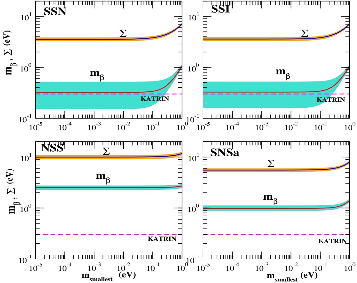
Figure 5: The sum of neutrino masses \Sigma and the kinematic neutrino mass m_\beta for scenarios SSN (top left), SSI (top right), NSS (bottom left) and SNSa (bottom right). The solid lines give the values of the respective observable at the best-fit point Eq. (4) while the shaded regions are obtained by varying the parameters involved in their corresponding ranges from Eqs. (3) and (6). We assumed that \Delta m_{s1}^2 = \Delta \tilde{m}_{s1}^2 and \Delta m_{s2}^2 = \Delta \tilde{m}_{s2}^2 . Scenario ISS is indistinguishable from case NSS, SISa is indistinguishable from SNSa, and SNSb/SISb are indistinguishable from NSS. For these two observables SSN and SSI give identical results. Also indicated is the KATRIN sensitivity on m_\beta of 0.3 eV.
