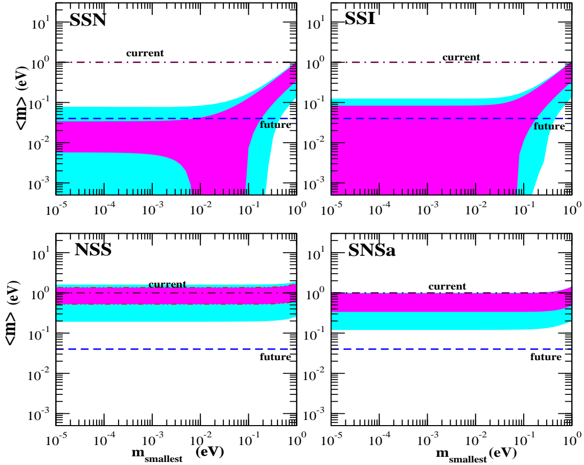
Figure 7: Same as Fig. 6 for the second typical sterile parameter point and the corresponding range from Eq. (5).
