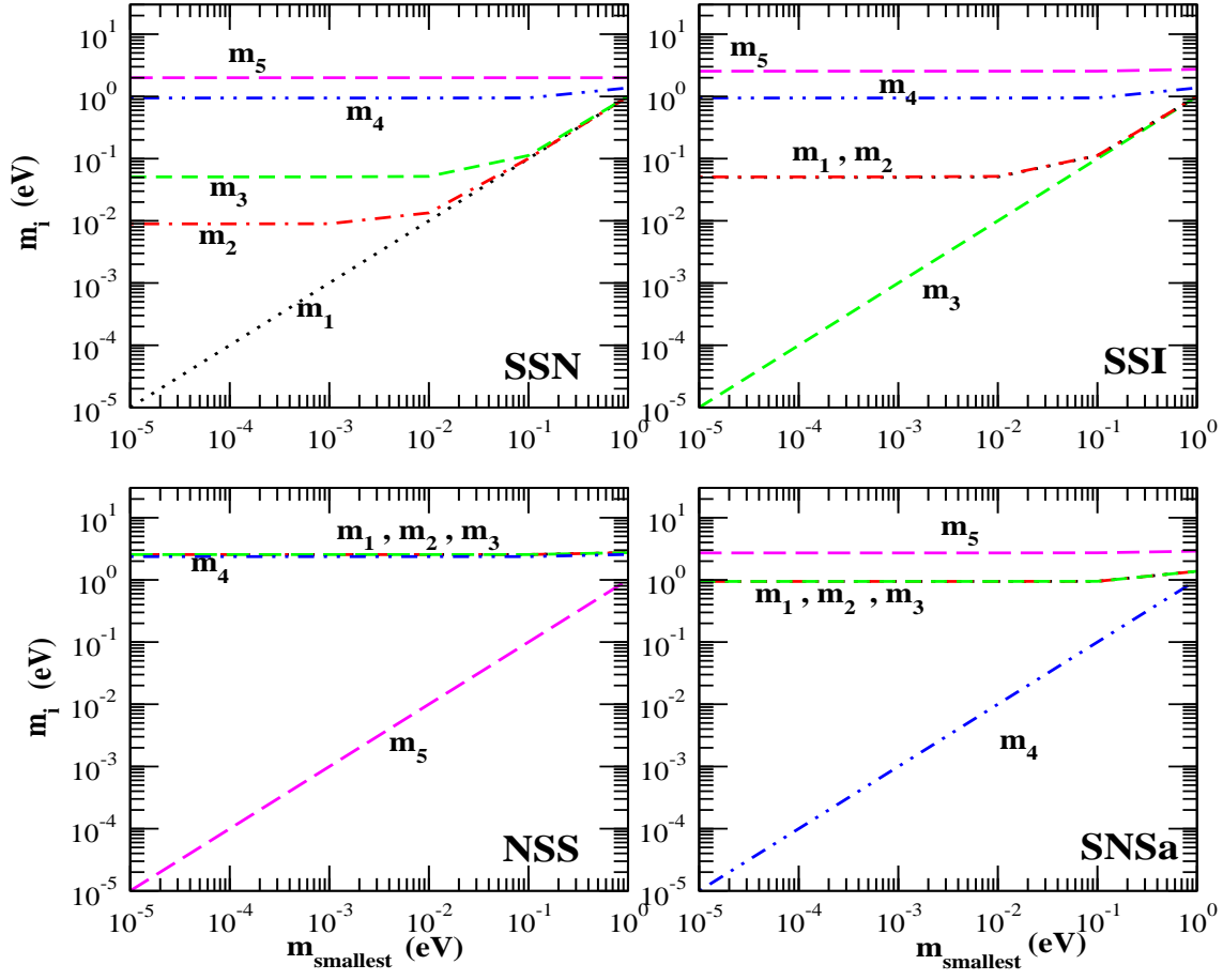
Figure 4: Scenarios with three active and two sterile neutrinos: the individual neutrino masses as a function of the smallest neutrino mass for scenarios SSN, SSI, NSS and SNSa. For the mass-squared differences related to the sterile neutrinos the best-fit point given in Eq. (4) is used and we assumed that \Delta m_{s1}^2 = \Delta \tilde{m}_{s1}^2 and \Delta m_{s2}^2 = \Delta \tilde{m}_{s2}^2 . Scenario ISS is indistinguishable from case NSS and SISa from SNSa. The schemes SNSb and SISb are very similar to NSS.
