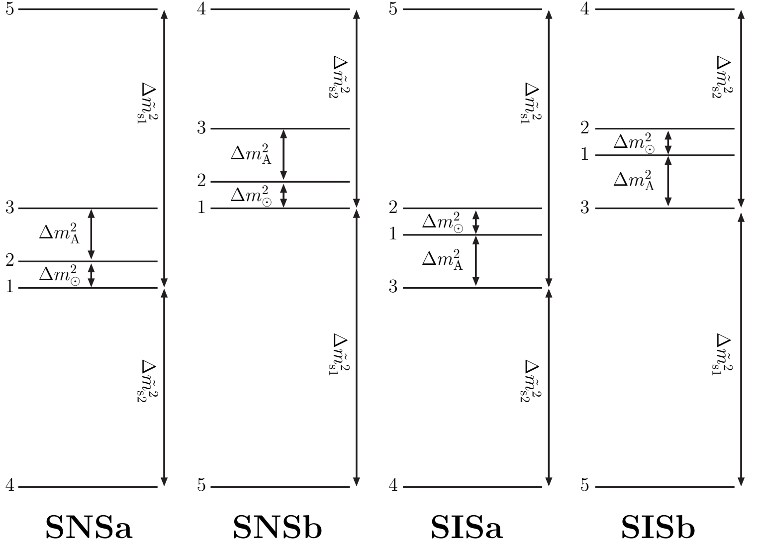
Figure 3: Allowed 1+3+1 mass orderings which are defined by having one sterile neutrino heavier than the three active ones which in turn are heavier than the second sterile neutrino. (Not to scale). Note that not necessarily \Delta \tilde{m}_{s1}^2 = \Delta m_{s1}^2 and \Delta \tilde{m}_{s2}^2 = \Delta m_{s2}^2 holds.
