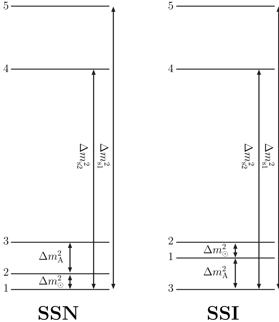
Figure 1: Allowed 2+3 mass orderings which are defined by having two sterile neutrinos heavier than the three active neutrinos. (Not to scale).
