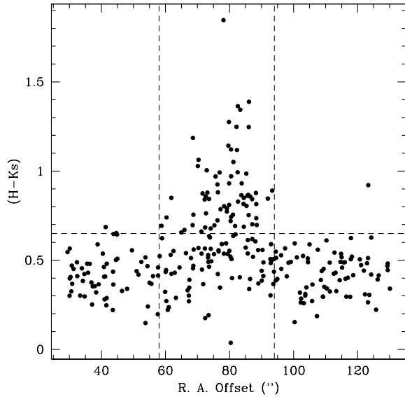
Fig. 4. Plot of the observed (H - K_s) colour of stellar sources as a function of the R. A. offset relative to the lower left (SE corner) of Fig. 3 (main panel). Sources closer than about 20 arcsec to the borders were excluded. The reddening effect ( (H - K_s) \geq 0.65 , horizontal dashed line) of a dense cloud core is clearly seen for values of R. A. offsets between approximately 58'' and 94'' (indicated by vertical dashed lines).
