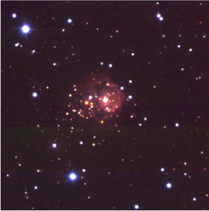
Fig. 2. J (blue), H (green), and Ks (red) colour composite image towards IRAS 06361-0142. The image covers about 70 \times 70 arcsec 2 . North is up and East to the left.
