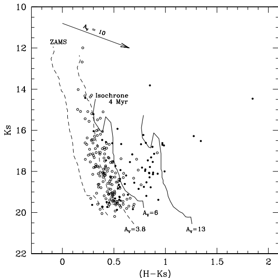
Fig. 6. Colour-magnitude diagram of the region towards IRAS 06361-0142 seen in Fig. 3. Filled circles and open circles have the same meaning as in Fig. 5. The two dashed lines are, respectively, the zero-age main-sequence (ZAMS) for an arbitrary distance with zero extinction and with A_v = 3.8 . The two solid lines are the 4 Myr isochrone with extinctions A_v = 6 and A_v = 13 . The reddening vector indicates the direction of the shift produced by extinction by dust with standard properties.
