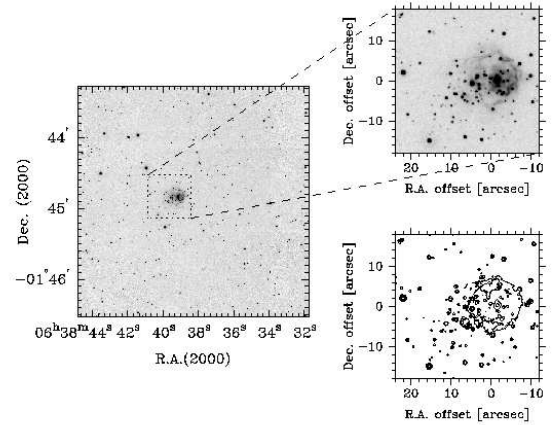
Fig. 3. Ks-band image towards IRAS 06361-0142. The close-up view at the top shows the central 36'' \times 36'' region (the “cluster region”). The close-up panel at the bottom shows the isophotes of the same region where the very close to circular shape of the extended nebulosity is evident. The axes give the coordinates relative to the estimated centre of the nebulosity, nearly coincident with the IRAS source (see text). The contour levels are at 5\sigma , 25\sigma , and 250\sigma above the sky level, where \sigma is the sky background noise in the central co-added region.
