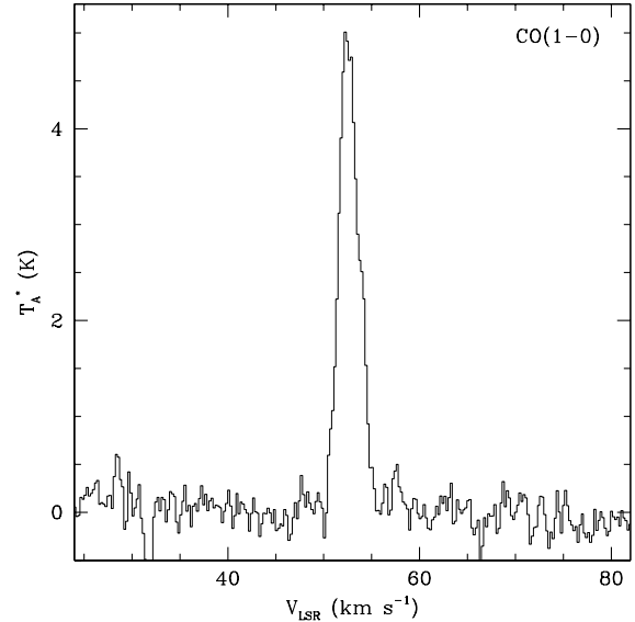
Fig. 1. CO ( J=1-0 ) spectrum towards IRAS 06361-0142 displaying a line at an LSR velocity of about 53 \text{ km s}^{-1} . The spectrum has been smoothed to a resolution of 0.22 \text{ km s}^{-1} .
