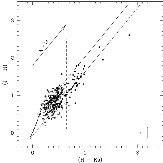
Fig. 5. Near-infrared colour-colour diagram of the region towards IRAS 06361-0142 seen in Fig. 3. Filled circles represent the 34 sources contained in the 36'' \times 36'' central region (“cluster region”, where most sources are likely to be members of the cluster – see text). Open circles are sources outside the cluster region. The solid line represents the locii of unreddened main-sequence stars, while long-dash lines indicate the reddening band. The reddening vector indicates the direction of the shift produced by extinction by dust with standard properties. The location of the vertical dotted line, derived from Fig. 4, is at (H - K_s) = 0.65 . The cross in the lower right corner represents the average error bars.
