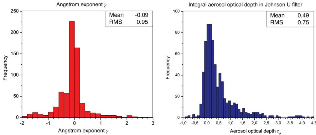
Figure 2: Histograms of measured distribution of Angstrom coefficient \gamma ( left ) and of integral aerosol optical depth \tau_A ( right ) for all data obtained from June 2006 until March 2007. Only the hardware quality cuts were applied, consequently some reconstruction artifacts are still apparent. For the aerosol optical depth distribution the left (negative) tail is due to mis-identified stars and the more prominent right tail ( \tau_A > 1 ) is due to observations through clouds.
