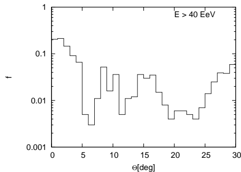
Figure 3: Fraction of simulations with larger number of pairs than the data for the 64 events with E > 40 EeV.
