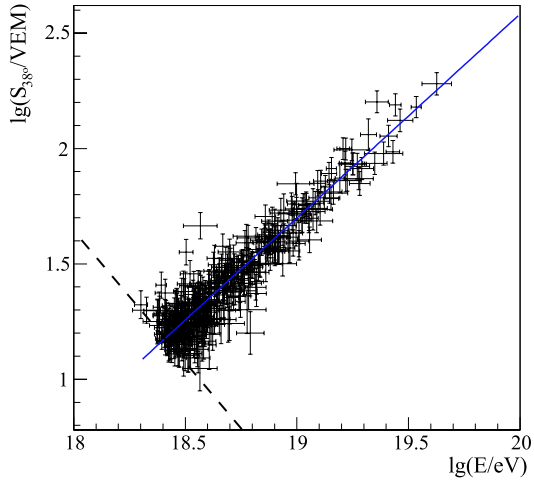
Figure 3: Correlation between \lg E_{FD} and \lg S_{38^\circ} for the 387 hybrid events used in the fit. The full line is the best fit to the data. Events below the dashed line were not included in the fit.
