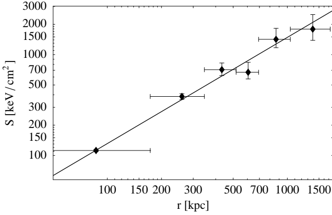
Fig. 4. Entropy as a function of radius and the best fit power law \log[S] = (1.053 \pm 0.005) \times \log[r] + (0.011 \pm 0.010) (entropy in \text{keV cm}^2 and radius in kpc).
