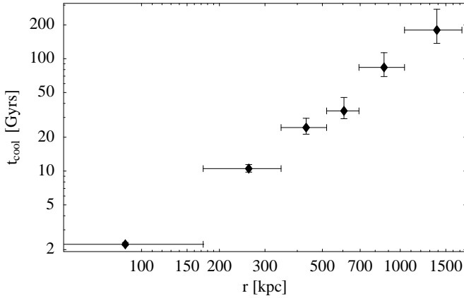
Fig. 3. Cooling time as a function of radius.
