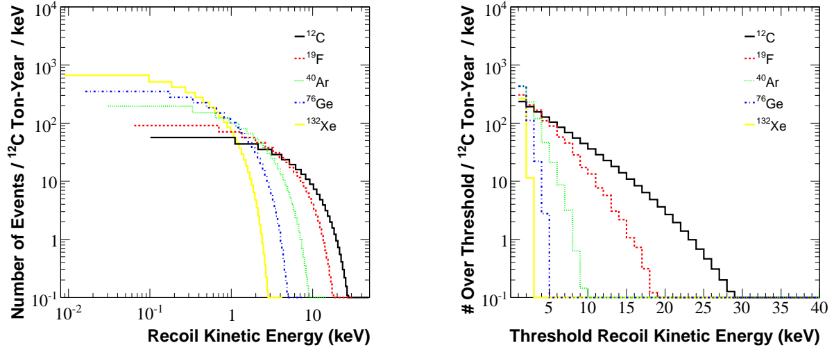
FIG. 4: Left: number of ^8B solar neutrino-nucleus coherent scattering events per ton-year exposure in various detector media, normalized per keV, vs. recoil kinetic energy (keV). Right: integrated number of neutrino-nucleus coherent scattering events above threshold per ton-year exposure in various detector media per keV vs. recoil kinetic energy threshold (keV) for ^8B solar neutrinos.
