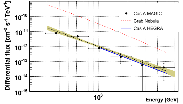
Fig. 3: Cas A spectrum above 250 GeV. The blue line represents the earlier measurement by HEGRA. The red line represents the Crab nebula spectrum. The shaded area is the 1\sigma statistical error of the fit.
