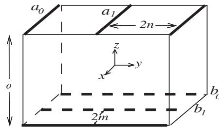
FIGURE 4. \text{Box}(G(m, n, o)) .
