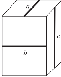
FIGURE 5. \text{Box}(H(p, q, r)) .
