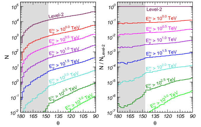
FIG. 1: (a) Expected zenith angle distribution of ATM \nu_\mu induced events in IceCube for different energy thresholds E_\mu^{\text{fin}, \min} for the PREM. \theta is the neutrino angle (which at these energies is collinear with the detected muon) as measured from the vertical direction (upgoing- \nu corresponding to \theta = 180 ). (b) Ratio of the zenith angle distribution of ATM \nu_\mu induced events in IceCube for different energy thresholds E_\mu^{\text{fin}, \min} over the corresponding one for L2 cuts only. The shadow areas cover the angular size of the Earth core.
