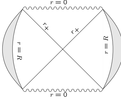
FIG. 3: Penrose-Carter diagram with two stellar objects connected by a Schwarzschild-de Sitter vacuum domain. Since the group orbits are decreasing at the matching surface the vacuum part contains the black hole horizon and the r = 0 singularity.
