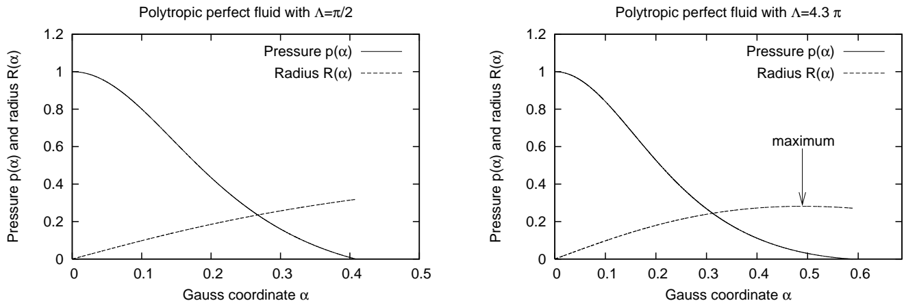
FIG. 4: Pressure function and radius for the polytropic equations of state, with K = 1 , n = 3 and \rho_b = 0.5 . Initial conditions are p_c = 1.0 ( \rho_c = 1.5 ) and \Lambda = \pi/2 (left), \Lambda = 4.3\pi (right).
