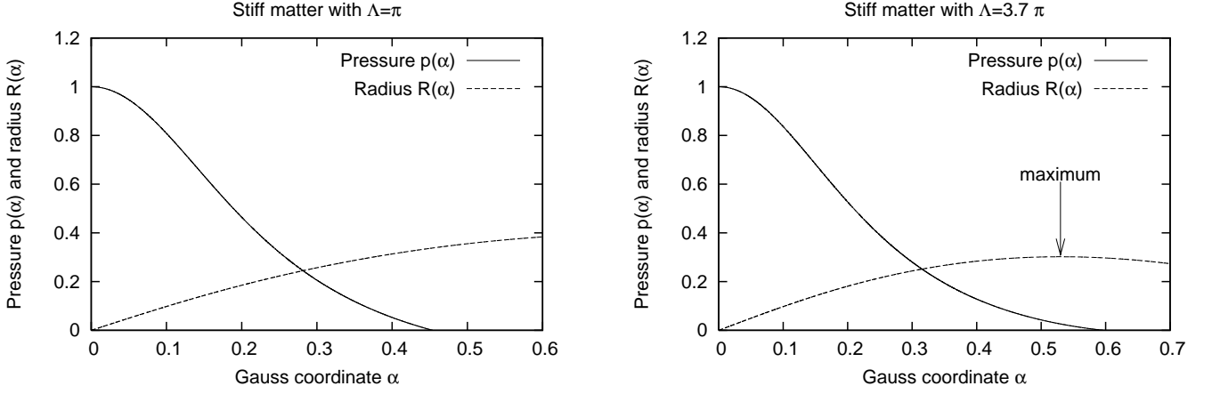
FIG. 5: Pressure function and radius for the stiff matter equation of state, with \rho_b = 0.5 . Initial conditions are p_c = 1.0 ( \rho_c = 1.5 ) and \Lambda = \pi (left), \Lambda = 3.7\pi (right).
