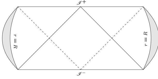
FIG. 2: Penrose-Carter diagram with two stellar objects having radii R which require the Nariai spacetime to be the vacuum part of the global solution. The solid and dashed lines represent the future and past event horizon, respectively.
