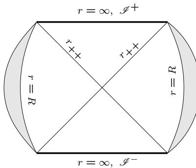
FIG. 1: Penrose-Carter diagram with two stellar objects separated by a Schwarzschild-de Sitter vacuum domain. The radii R of the stellar objects is between the radii of the black hole and cosmological horizons. Since the group orbits are increasing up to R the vacuum part contains the cosmological event horizon r_{++} .
