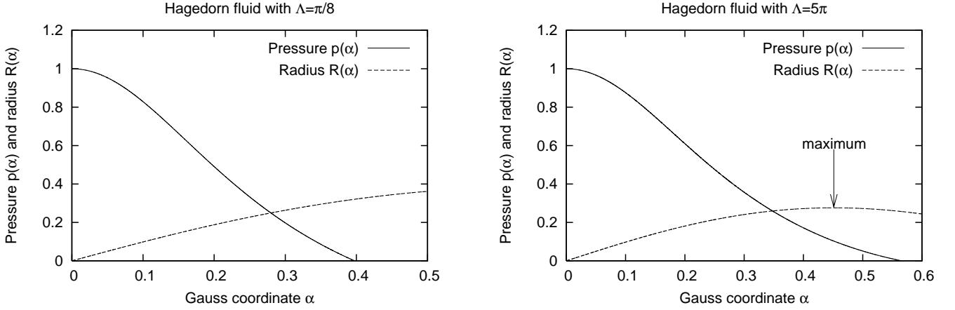
FIG. 6: Pressure function and radius for the Hagedorn equation of state, with \rho^* = 2.0 . Initial conditions are p_c = 1.0 ( \rho_c \approx 1.21 ) and \Lambda = \pi/8 (left), \Lambda = 5\pi (right).
