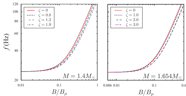
Figure 2. With M = 1.4M_{\odot} and 1.654M_{\odot} , the frequencies of the fundamental torsional modes of \ell = 2 as functions of B/B_{\mu} , where B_{\mu} = 4 \times 10^{15} Gauss. The different lines correspond to different values of \zeta , where \zeta_{max} \sim 1.9 for M = 1.4M_{\odot} and \zeta_{max} \sim 3.0 for M = 1.654M_{\odot} .
