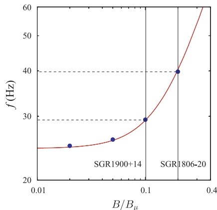
Figure 3. The torsional mode frequencies as functions of the magnetic field strength for \zeta = 0 . The continuous line shows the results from the 1-D truncated mode calculation on which we omitted the coupling to \ell \pm 2 equations while the thick dots correspond to results from 2D numerical evolutions of the perturbation equations. In this figure two vertical lines has been drawn corresponding to the estimated magnetic field strengths for the two SGRs that is B \approx 4 \times 10^{14} Gauss for SGR 1900+14 and B \approx 8 \times 10^{14} Gauss for SGR 1806-20.
