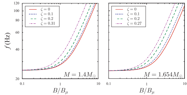
Figure A2. The frequencies of the fundamental torsional modes with \ell = 2 as functions of B/B_\mu with M = 1.4M_\odot and 1.654M_\odot . The different lines correspond to different values of \zeta , where \zeta_{max} \sim 0.31 for M = 1.4M_\odot and \zeta_{max} \sim 0.27 for M = 1.654M_\odot .
