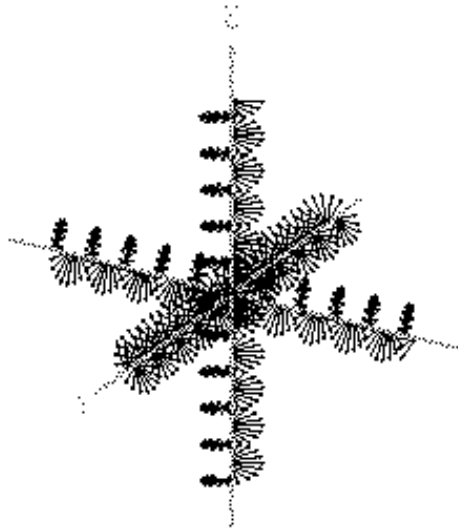
Figure 13: Cartan's spiral staircase , see García et al. [22]. Cartan's rules [12] for the introduction of a non-Euclidean connection in a 3D Euclidean space are as follows: (i) A vector which is parallelly transported along itself does not change (cf. a vector directed and transported in x -direction). (ii) A vector that is orthogonal to the direction of transport rotates with a prescribed constant "velocity" (cf. a vector in y -direction transported in x -direction). The winding sense around the three coordinate axes is always positive.
