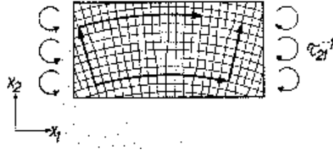
Figure 11: Deformation of a cubic crystal by edge dislocations of type \alpha_{12}^1 : The relative orientations of the lattice plains in 2-direction change. A vector in x_2 -direction will rotate, if parallelly displaced along the x_1 -direction. As a consequence a contortion \kappa_{112} emerges and the closure failure occur of the “infinitesimal” parallelogram.
