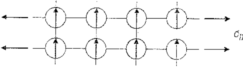
Figure 3: Conventional homogeneous strain \varepsilon_{11} of a Cosserat continuum: Distance changes of the “particles” caused by force stress \sigma_{11} .
