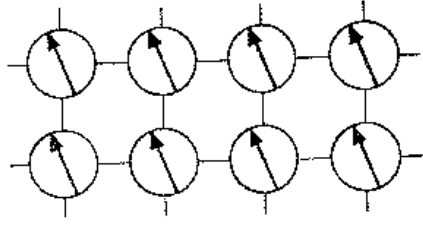
Figure 5: Homogeneous Cosserat rotation \omega_{12} of the “particles” of a Cosserat continuum caused by the antisymmetric piece of the stress \Sigma_{[12]} .
