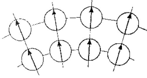
Figure 6: Conventional rotation \partial_{[1}u_{2]} of the “particles” of a Cosserat continuum caused by an inhomogeneous strain.
