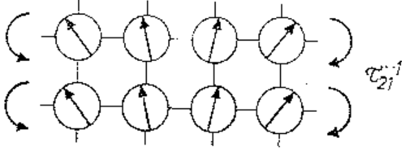
Figure 4: Homogeneous contortion \kappa_{112} of a Cosserat continuum: Orientation changes of the “particles” caused by spin moment stress \tau_{21}^1 .
