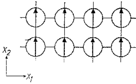
Figure 2: Schematic view on a two-dimensional Cosserat continuum: Undeformed initial state.
