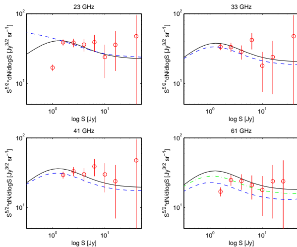
Figure 4. Differential number counts, in bins of \Delta \log(S) = 0.2 , multiplied by S^{0.5} , of the NEWPS _{5\sigma} sources (circles with Poisson error bars). The solid curve shows, for comparison, the total counts predicted by the De Zotti et al. (2005) model. The dashed lines correspond to the counts extrapolated from 5 GHz, for the 23 GHz case, and from 23 GHz for the other frequencies, using the spectral index distributions of § 4.1. The extrapolated counts are too low at 61 GHz, suggesting that the true steepening of spectral indices above 23 GHz is less pronounced than implied by the distribution yielded by the Kaplan-Meier estimator. A good fit is obtained damping down the secondary peak of the distribution of \alpha_{23}^{61} (Fig. 2) by a factor of 0.2 (dot-dashed line).
