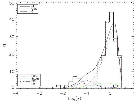
Figure 1. Redshift distributions of the full |b| > 10^\circ sample, of QSOs and of galaxies (solid, dashed, and dot-dashed histograms, respectively). The dotted, dashed, and dot-dashed curves display, for comparison, the predictions of the model by De Zotti et al. (2005) for Flat-Spectrum Radio QSOs, BL Lacs, Fanaroff-Riley type II sources, while the solid line shows the total.
