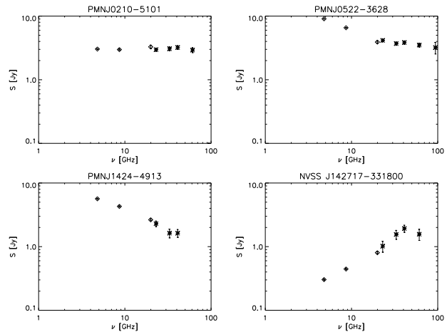
Figure 3. Examples of typical radio source spectra at mm wavelengths: a flat-spectrum source ( top left panel ); a steep-spectrum source ( bottom left panel ); a source whose spectrum flattens at \nu \sim 10 GHz ( top right panel ); a High Frequency Peaker (HFP) source ( bottom right panel ). Data from the NEWPS Catalogue ( asterisks ) and from the AT20G Survey (courtesy of the AT20G group, Massardi et al. (in preparation)) ( diamonds ).
