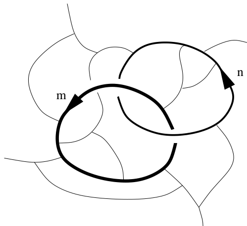
FIG. 1: The elements of a natural basis of the kinematical Hilbert can be written as the product of: 1) A functional of the Lorentz connection labelled by a graph in space and the assignment of unitary irreducible representations of the Lorentz group, i.e., a SO(3, 1) spin-network state (represented by the thin-lines graph), 2) An n -point spin function (represented here by the endpoints of the thin-lines-graph on the strings; see [7] for the precise definition), 3) A functional of the Yang-Mills connection given by the product of Wilson loops on a unitary representation of the structure group G along the each string component.
