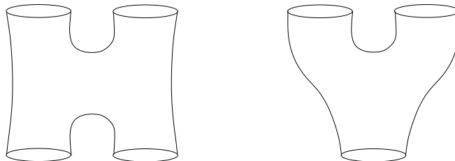
FIG. 2: Interacting string world sheets
