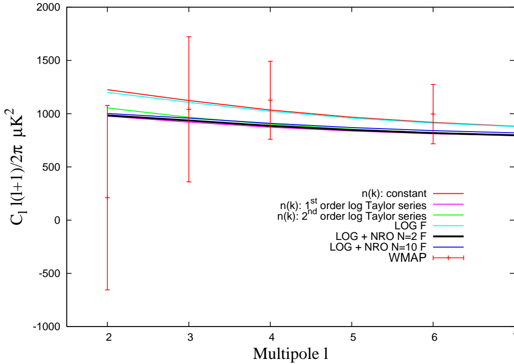
Figure 4: CMB temperature power spectrum for the best-fit model parameters for the standard parametrization, the LOG and the LOG+NRO scenarios. The bottom panel shows the details of the large-scale region.
