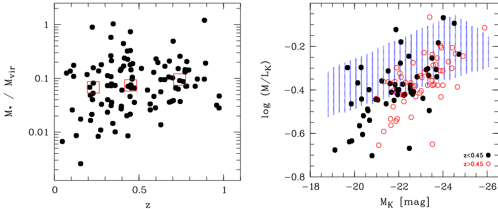
Figure 1. left: The observed stellar mass fraction is roughly constant at redshifts 0 < z < 1 (squares give median values in three z -bins). right: Stellar mass-to-light ratios of our sample at 0.1 < z < 0.45 (filled circles) and 0.45 < z < 1.0 (open circles), compared to the parameter range covered by present-day spirals (shaded area) from Bell & de Jong (2001). The data indicate a stronger evolution in stellar M/L for low-luminosity disk galaxies.
