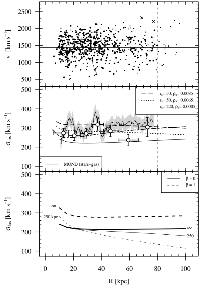
Fig. 1. Kinematics of GCs around NGC 1399. The upper panel shows the radial velocities of our total sample versus the radial distance, where 80 kpc correspond to 14.5 arcmin. The two crosses are outlier velocities that we have discarded, and the larger points show objects from the “safe” sample. The horizontal line marks the systemic velocity, and the vertical dashed line indicates the radial limit used for the “safe” sample. The middle panel shows the velocity dispersion profile. The thin solid line with shaded region shows the result derived for the full GC sample along with its uncertainties, while the circles with error bars show the “safe” sample. The curves represent various dynamical model fits (isotropic), as described in the text, and with parameters summarized in the legend. The lower solid line represents the expectation from MOND under isotropy. The lower panel shows in addition fully radial MOND models (without gas) with a cut-off radius of 250 kpc.
