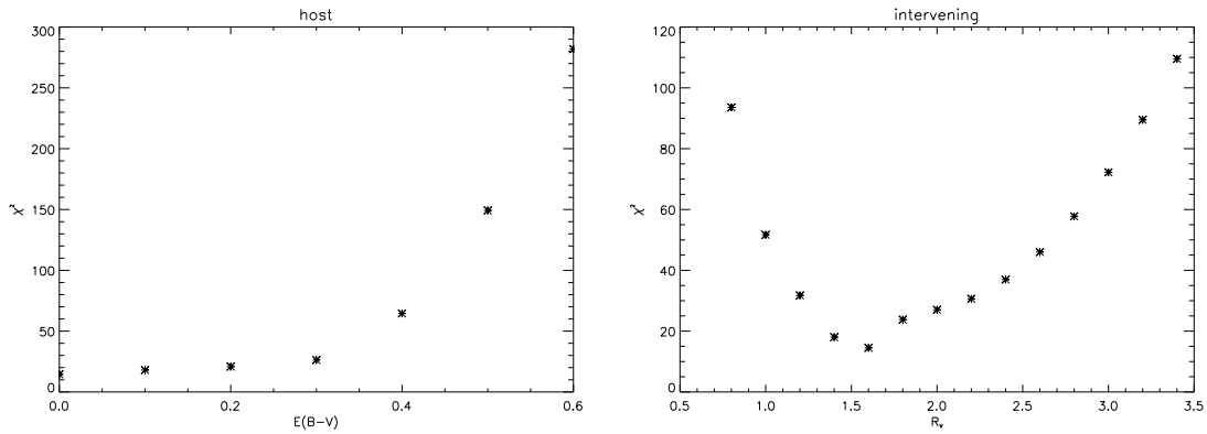
Fig. 9. The \chi^2 values for different E(B - V) in the host galaxy (first panel) and R_V in the intervening galaxy (second panel) for MG0414+0534.
