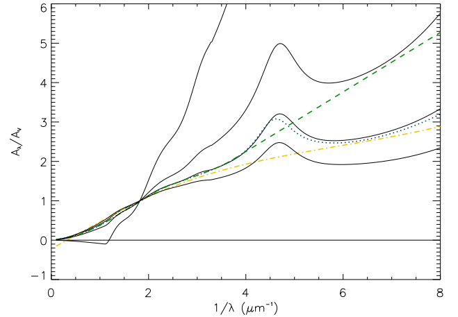
Fig. 1. The CCM parameterisation of the Milky Way extinction curve (solid black line) for four different R_V (0.5, 2, 3.1 and 4) where the highest values of R_V correspond to the flattest curves. We also show the Fitzpatrick parameterisation (dotted blue) with R_V = 3.1 , the Prévot law for SMC-like extinction (dashed green) with R_V = 3.1 and the starburst extinction law (dashed dotted yellow) with the preferred value for starburst galaxies R_V = 4.05 (Calzetti et al. 2000). A_\lambda is the extinction at wavelength \lambda and A_V is the visual extinction.
