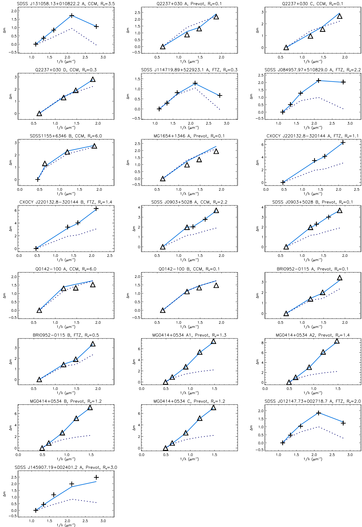
Fig. 5. Comparison of the measured magnitudes (black signs) with the fitted magnitudes (light blue solid line) for the images that could be fitted using the dust laws. The dark blue dotted line shows the expected magnitudes without dust. Note that sometimes only one line is visible when the best fit is with little or no extinction. The ground-based measurements are marked with plus signs while the HST observations are marked with triangles. All magnitudes are normalised so that the magnitude at the longest wavelength is zero.
