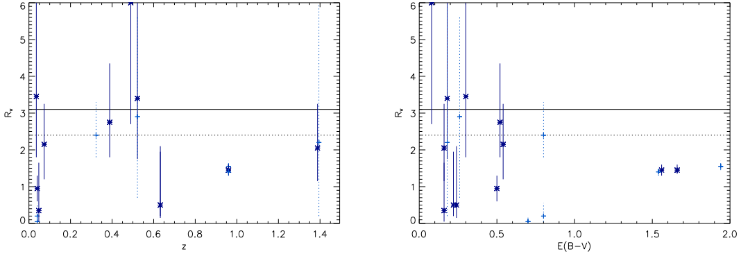
Fig. 8. The fitted values of R_V with the 1\sigma errorbars for all images that could be fitted using the Fitzpatrick parameterisation of dust in an intervening galaxy. The first panel shows R_V as a function of dust redshift and the second as a function of colour excess. In the first panel, the results from the different images of the same quasar will be plotted on top of each other since they all have the same redshift. In the second panel, the results of different images will be plotted in different places along the x axis since E(B - V) differs at least slightly between the images. The fitted values which have a larger probability than 10% (see Table 3) are plotted with stars and dark blue solid errorbars while the less reliable ones, with a smaller probability than 10%, are plotted with plus signs and dotted light blue errorbars. The most probable value of R_V found when co-adding the probability distributions for the fits (see Figure 7) is indicated with a dotted line at R_V = 2.4 .
