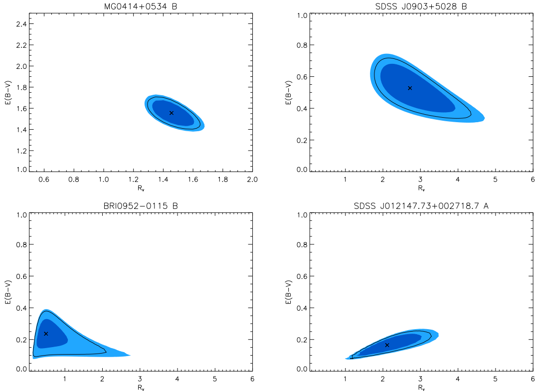
Fig. 4. Confidence levels for some of the quasar images that could be fitted by dust extinction in the intervening galaxy using the Fitzpatrick extinction law. The levels correspond to 1\sigma for one parameter (black line) and 68% (dark blue region) and 90% (pale blue) for two parameters.
