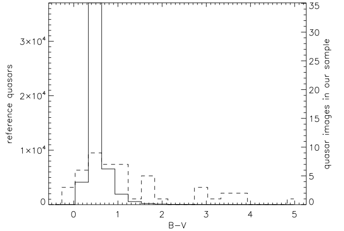
Fig. 2. A histogram over rest-frame B - V for the quasars in SDSS DR3 (solid line), and for the quasar images in our sample (dashed line).
