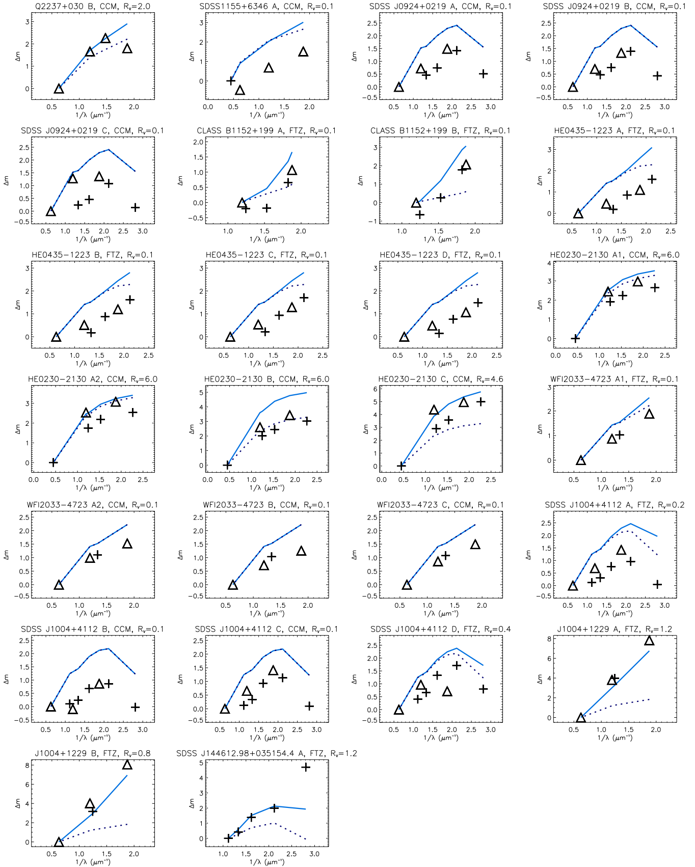
Fig. 6. Comparison of the measured magnitudes (black signs) with the fitted magnitudes (light blue solid line) for the images that were badly fitted using the dust laws. The dark blue dotted line shows the expected magnitudes for no extinction. Note that sometimes only one line is visible when the best fit is with little or no extinction. The ground-based measurements are marked with plus signs while the HST observations are marked with triangles. All magnitudes are normalised so that the magnitude at the longest wavelength is zero.
