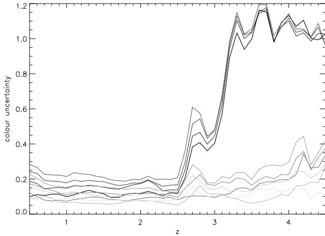
Fig. 3. Uncertainties in the template colours for u-g , u-r , u-i , u-z , g-r , g-i , g-z , r-i , r-z , i-z (from black to light grey) as a function of redshift z .
