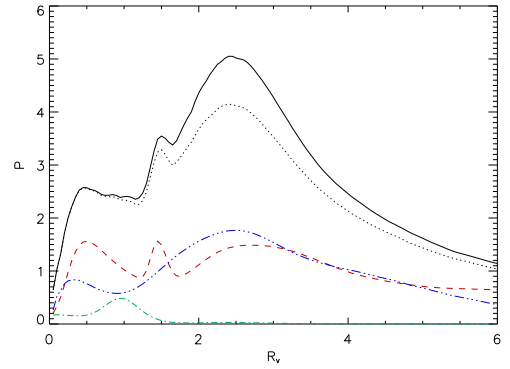
Fig. 7. The co-added probability distributions for the fits with intervening dust following the Fitzpatrick extinction law, weighted by the probability of the fit. The dotted line shows the added probability when using the well fitted quasar images in Table 3 and the solid line when also the objects in Table 4 are included. The added probabilities for the subset of early-type galaxies (dashed line), late-type galaxies (dash-dot) and starburst/star-forming galaxies (dash-dot-dot-dot) are also included in the figure.
