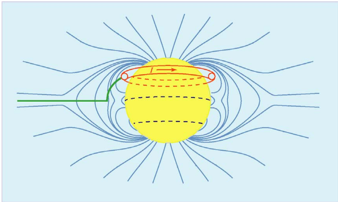
Figure 6. Field lines of the solar global magnetic field typical for minimum activity adopted in the axially-symmetric flux rope model (Filippov et al., 2002). The dashed lines show the polarity inversion lines at the photospheric surface, and the green line, the possible equilibrium positions of the flux rope.
