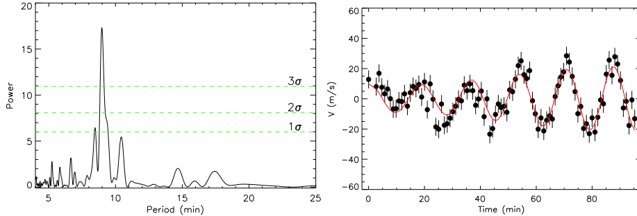
Figure 1. Left panel: Periodogram showing discovery of 9-min pulsational signal in the combined RVs of 29 Nd III lines in HD 75445. Right panel: Mean RV variation of 40 Ce II lines in \beta CrB. Multiperiodic character of oscillation is clearly evident.
