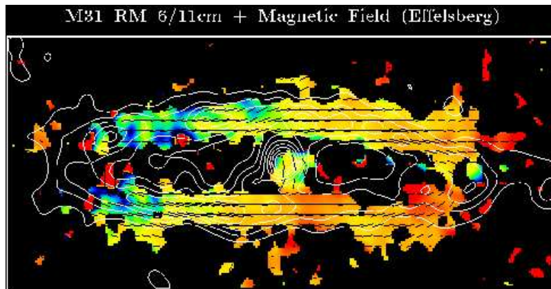
Figure 1: M 31: total emission (contours) and polarized emission (B-vectors) at \lambda 6.2 cm superimposed with the distribution of the Faraday rotation measure from diffuse radio emission [5].
