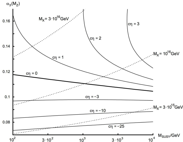
FIG. 1: For \eta fixed by the particle content of the theory, solid lines are contours of constant c such that, under the presence of the gravitationally induced and enhanced operator (5), SUSY-SU(5) perfectly unifies at two loops for given values of the initial strong coupling constant \alpha_3(M_Z) and SUSY breaking scale M_{\text{SUSY}} . Over the whole range, unification happens for some value of the coefficient c , with unification scale and unified coupling between M_X = 9.3 \times 10^{14} GeV, \alpha_G = 0.033 (lower right corner) and M_X = 5.5 \times 10^{16} GeV, \alpha_G = 0.045 (upper left).
