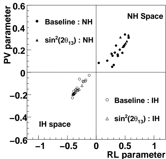
FIG. 3: Distribution of RL and PV values for different parameters of baseline and \sin^2(2\theta_{13}) . For each parameter to be scanned, the default baseline is 60 km and all the other parameters are the values as in Table I. Two clusters of RL and PV values are clearly seen for NH and IH cases.
