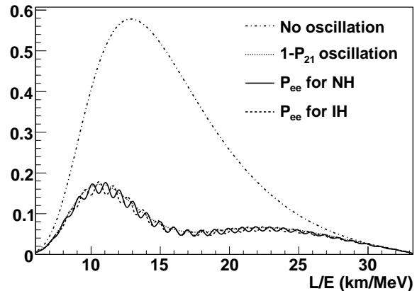
FIG. 1: Reactor neutrino spectra at a baseline of 60 km in L/E space for no oscillation (dashed dotted line), 1 - P_{21} oscillation (dotted line) and P_{ee} oscillation in the cases of NH and IH, assuming \sin^2(2\theta_{13}) = 0.1 .
