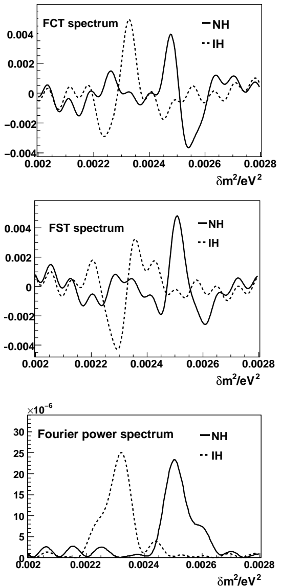
FIG. 4: The FCT and FST spectra and Fourier power spectrum for \sin^2(2\theta_{13}) = 0.005 . The solid line is for NH and the dashed line is for IH. The FCT and FST spectra have distinctive features to identify the mass hierarchy, which looks more sensitive than the Fourier power spectrum method.
