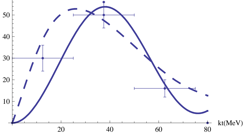
Figure 1: The differential cross-section \frac{d\sigma}{dyd^2k_{\perp}} for y=0 calculated in ADS as a function of transverse meson momentum k_{\perp} (solid line) compared against the photon-pomeron fusion calculation of Hencken et al (dashed line). 16 . The vertical scale is chosen arbitrarily as normalizations cannot be calculated in our model. Also shown are data points from the Star Collaboration 12 for the number of \rho^0 counts, binned in 25 MeV intervals.
