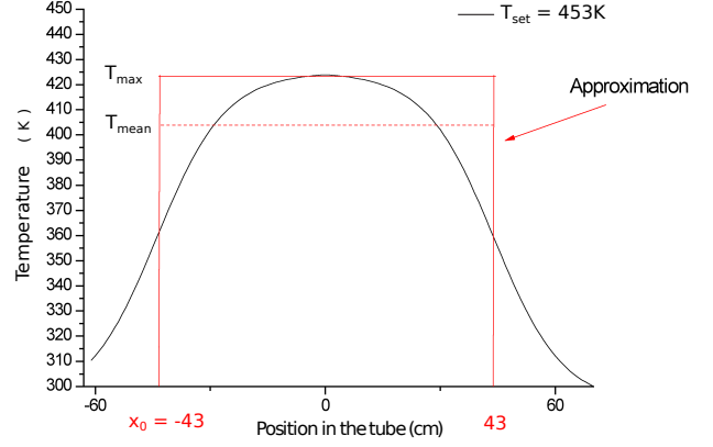
Fig. 5: Temperature inside the absorption cell for T_{set} = 453 K. The maximum temperature T_{max} is 420 K and the mean temperature T_{mean} is (410 \pm 15) K. The portion of gas out of the range [-x_0; x_0] is considered at ambient temperature.
