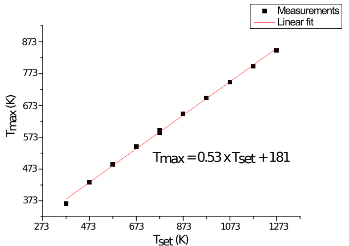
Fig. 2: Relation between the set temperature ( T_{set} ) and the temperature measured at the center of the oven ( T_{max} ).
