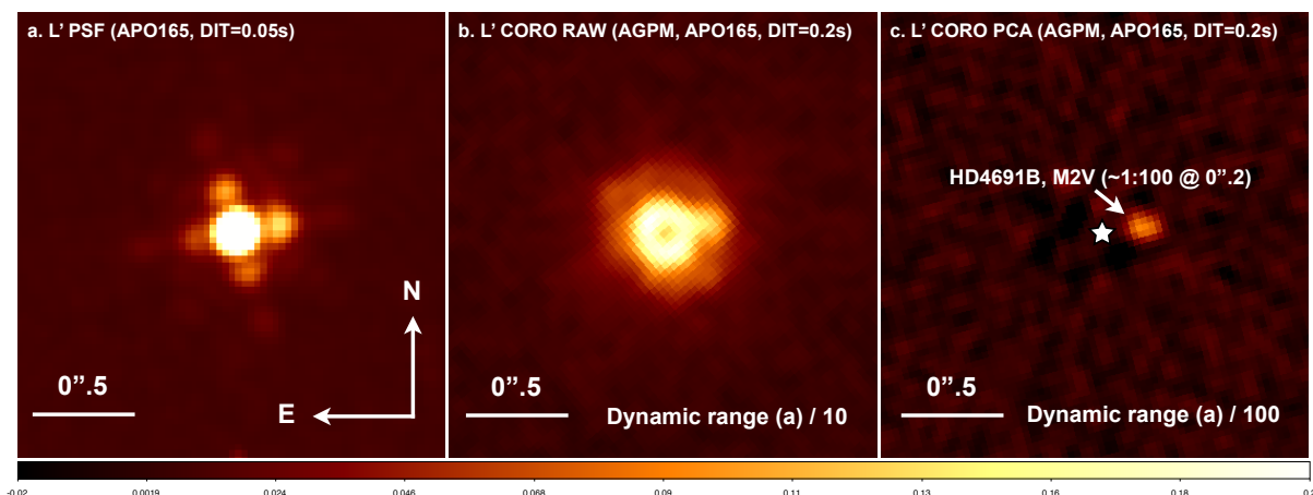
Fig. 3. a: L'-band NACO PSF with the APO165 pupil mask in the beam. b: L'-band NACO coronagraphic image with the star centered on the AGPM (the dynamic range and corresponding colorbar/scale are a factor of 10 smaller than in image a). c: Result of our PCA-ADI data reduction pipeline, revealing a putative faint off-axis M2V companion at only \approx 0''.19 (the dynamic range and corresponding colorbar/scale are a factor of 100 smaller than in image a). The scale is linear on all images (and scaled down by a factor of 10 and 100 for b and c, respectively), illustrating in sequence the benefits of coronagraphy and optimized data reduction technique. The bottom color bar refers to Figure a.
