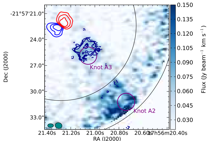
Fig. 4. CO J=3-2 integrated intensity map of the blue shifted wind from HD 163296. The colourscale shows the primary beam corrected integrated intensity of the J=3-2 emission. The black, blue and red circles and contours are the same as Figure 2. The molecular counterpart to HH knot A2 is more prominent in this image because we have corrected for the fall-off in sensitivity as a function of distance from the pointing center.
