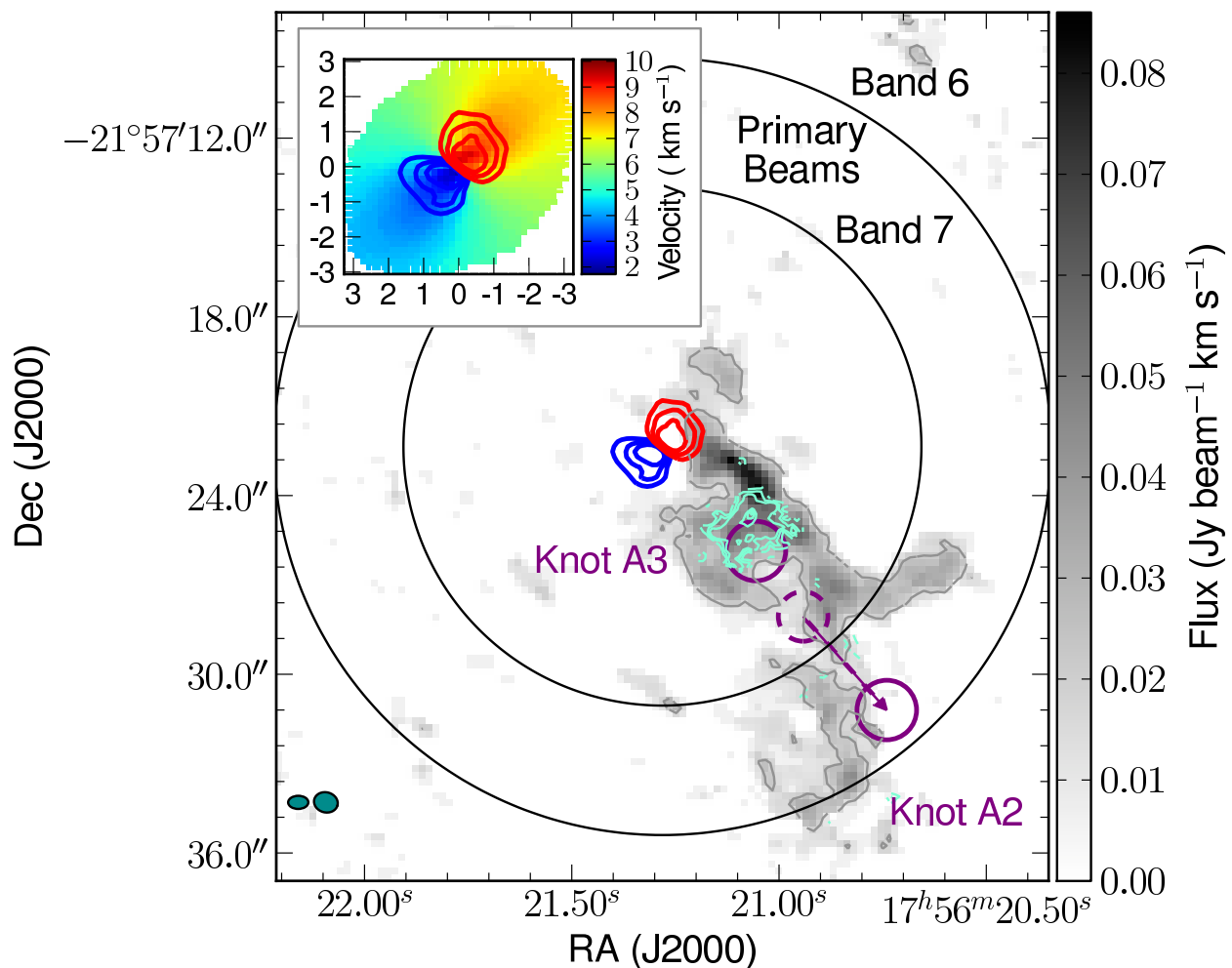
Fig. 2. Blue shifted disk wind from HD 163296. The greyscale and single ( 4\sigma ) contour show the CO J=2-1 integrated intensity of the blue shifted wind from HD 163296. The blue and red contours show the 15, 20 and 25 times the rms noise ( 20 \text{ mJy beam}^{-1} ) of the blue ( -2 to 5.5 \text{ km s}^{-1} ) and red ( 6 to 12 \text{ km s}^{-1} ) \text{HCO}^+ J=4-3 emission in the disk. The inset image shows the first moment map of the \text{HCO}^+ J=4-3 emission in the disk, with the same red and blue contours as in the main figure for reference. The two black arcs show the primary beams of the 345 GHz (smaller) and 230 GHz (larger) observations. The cyan contours show 4, 6, and 8 times the rms noise in the CO J=3-2 emission ( 2.6 \text{ mJy beam}^{-1} ). The two solid purple circles show the 2012 positions of knots A2 and A3 as described in the text. The dashed purple circle and arrow show the position of knot A2 in 2004, and its projected motion to 2012. The two dark cyan circles in the bottom left corner show the synthesized beams of the Band 7 (left) and Band 6 (right) datasets. The dimensions of the synthesized beams are given in Table 1.
