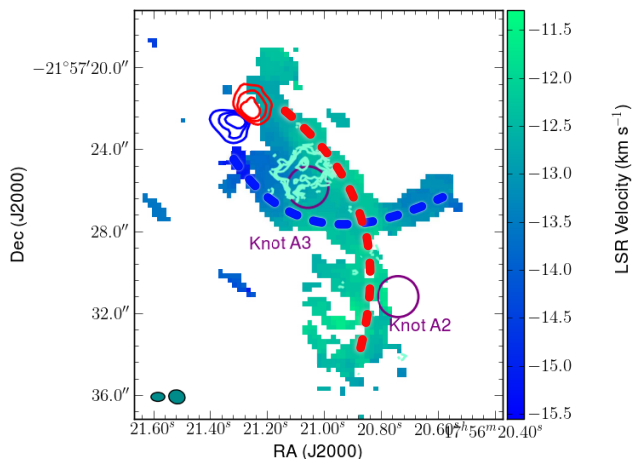
Fig. 3. CO J=2-1 intensity weighted velocity map of the blue shifted wind from HD 163296. The purple circles show the 2012 positions of the knots, the blue and red contours show the \text{HCO}^+ J=4-3 emission, and the two dark cyan circles in the bottom left corner show the synthesized beams of the observations, as in Figure 2. The blue and red dashed lines delineate the double corkscrew described in the text.
