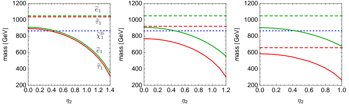
Figure 1: Plot of the \tilde{\tau}_1 (red, solid lines) and \tilde{e}_1 (green, solid lines) mass vs. \eta_2 coupling for \tan\beta = 10 (left plot), \tan\beta = 30 (middle plot) and \tan\beta = 50 (right plot). Blue, dotted lines represent mass of lightest neutralino (bino). h_{14} is set to 1.2, while \xi scale is 1.6 \times 10^5 GeV. Dashed lines show masses of the particles when h_{14} = \eta_2 = 0 , which corresponds to the standard GMSB case. The plots are symmetric under \eta_2 \rightarrow -\eta_2 because of m_{\tilde{Q},\eta}^2 \sim \eta_2^2 . In this case \tilde{\tau}_1 and \tilde{e}_1 are mostly right-handed.
