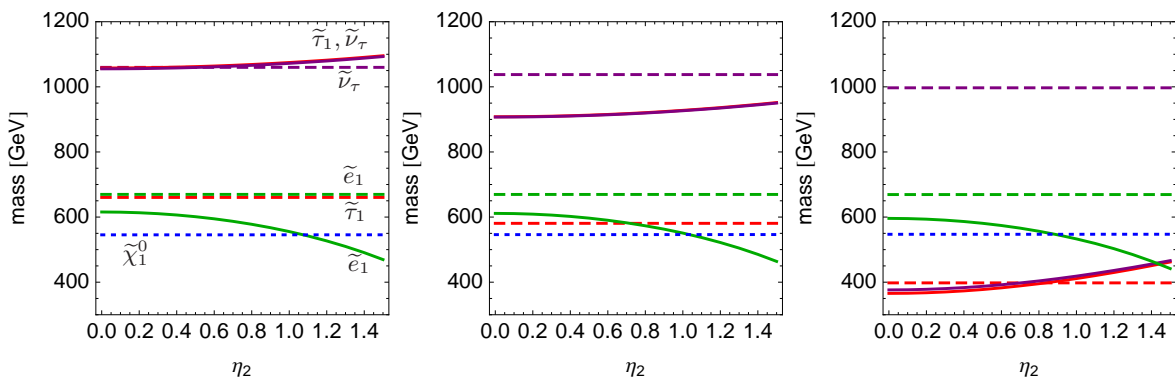
Figure 2: Plot of the \tilde{\tau}_1 (red, solid lines), \tilde{e}_1 (green, solid lines) and \tilde{\nu}_\tau (purple, solid lines) mass vs. \eta_2 coupling for \tan\beta = 10 (left plot), \tan\beta = 30 (middle plot) and \tan\beta = 50 (right plot). Blue, dotted lines represent mass of lightest neutralino (bino). The \xi scale is chosen to be 10^5 GeV. h_8 and h_{11} are fixed to 0.9 and 0.6, respectively, what results in m_{h^0} \approx 125 GeV. Dashed lines show masses of the particles when h_8 = h_{11} = \eta_2 = 0 , which corresponds to the standard GMSB case. The plots are symmetric under \eta_2 \rightarrow -\eta_2 because of m_{H_u, \eta}^2 \sim \eta_2^2 . Selectron and tau sneutrino masses are nearly degenerated. Here \tilde{e}_1 is mostly right-handed, while \tilde{\tau}_1 is mostly left-handed.
