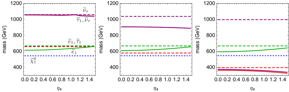
Figure 3: Plot of the \tilde{\tau}_1 (red, solid lines), \tilde{e}_1 (green, solid lines) and \tilde{\nu}_\tau (purple, solid lines) mass vs. \eta_4 coupling for \tan\beta = 10 (left plot), \tan\beta = 30 (middle plot) and \tan\beta = 50 (right plot). Blue, dotted lines represent mass of lightest neutralino (bino). The \xi scale is chosen to be 10^5 GeV. h_8 and h_{11} are fixed to 0.9 and 0.6, respectively, what results in m_{h^0} \approx 125 GeV. Dashed lines show masses of the particles when h_8 = h_{11} = \eta_4 = 0 , which corresponds to the standard GMSB case. The plots are symmetric under \eta_4 \rightarrow -\eta_4 because of m_{Q,\eta}^2 = m_{U,\eta}^2 \sim \eta_4^2 . Selectron and tau sneutrino masses are nearly degenerated. Here \tilde{e}_1 is mostly right-handed, while \tilde{\tau}_1 is mostly left-handed.
