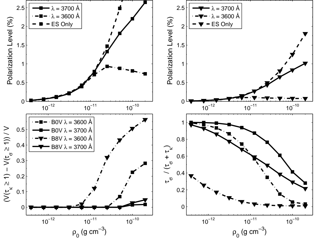
Fig. 12.— Top left: Polarization levels for a B0V star. Top right: Polarization levels for a B8V star. Bottom left: Size of the effective absorbing volume minus the effective scattering volume. Bottom right: Equatorial electron scattering optical depth with respect to the total equatorial optical depth. The modelled stars are viewed at an inclination of i = 75^\circ and surrounded by a disk with n = 3.5 and with \rho_0 increasing from 3.81 \times 10^{-13} \text{ g cm}^{-3} to 2.0 \times 10^{-10} \text{ g cm}^{-3} .
