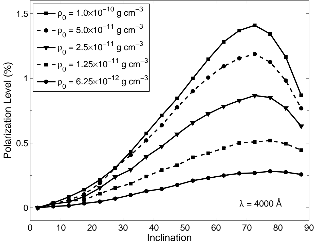
Fig. 3.— Polarization level versus inclination for a B2V star with circumstellar disks with varying \rho_0 and n = 3.5 . For all the values of \rho_0 plotted, the polarization level peaks between i = 70^\circ and i = 80^\circ .
