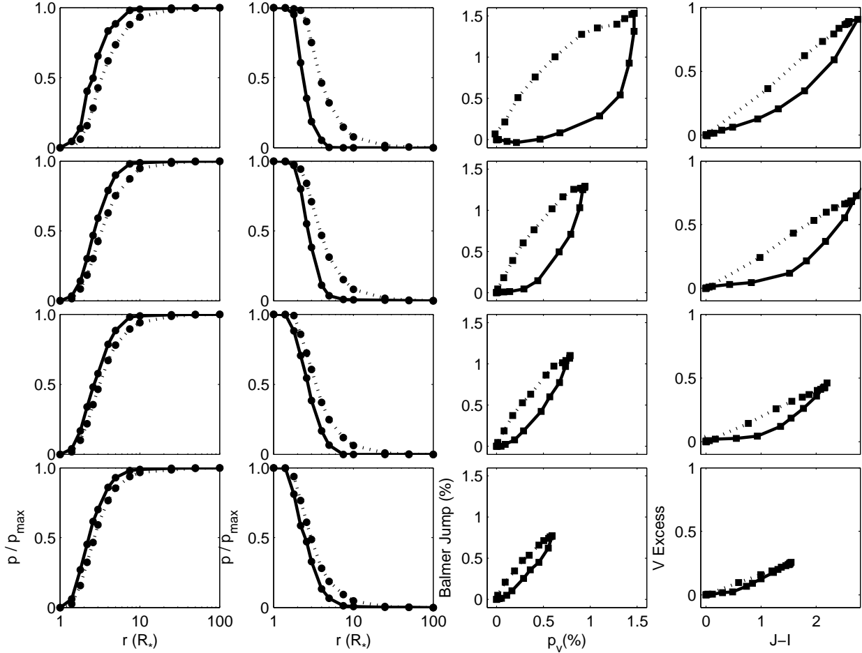
Fig. 10.— Column 1: Balmer jump (solid line) and V-band polarization level (dotted line) during disk growth. Column 2: Balmer jump (solid line) and V-band polarization level (dotted line) during disk dissipation. Column 3: BJV diagram at i = 75^\circ showing disk growth (dotted line) and dissipation (solid line). Column 4: Color magnitude diagram at i = 15^\circ showing disk growth (dotted line) and dissipation (solid line). From top to bottom: B0V, B2V, B5V and B8V stars. The models correspond to disks with n = 3.5 and with \rho_0 = 1.0 \times 10^{-10} \text{ g cm}^{-3} .
