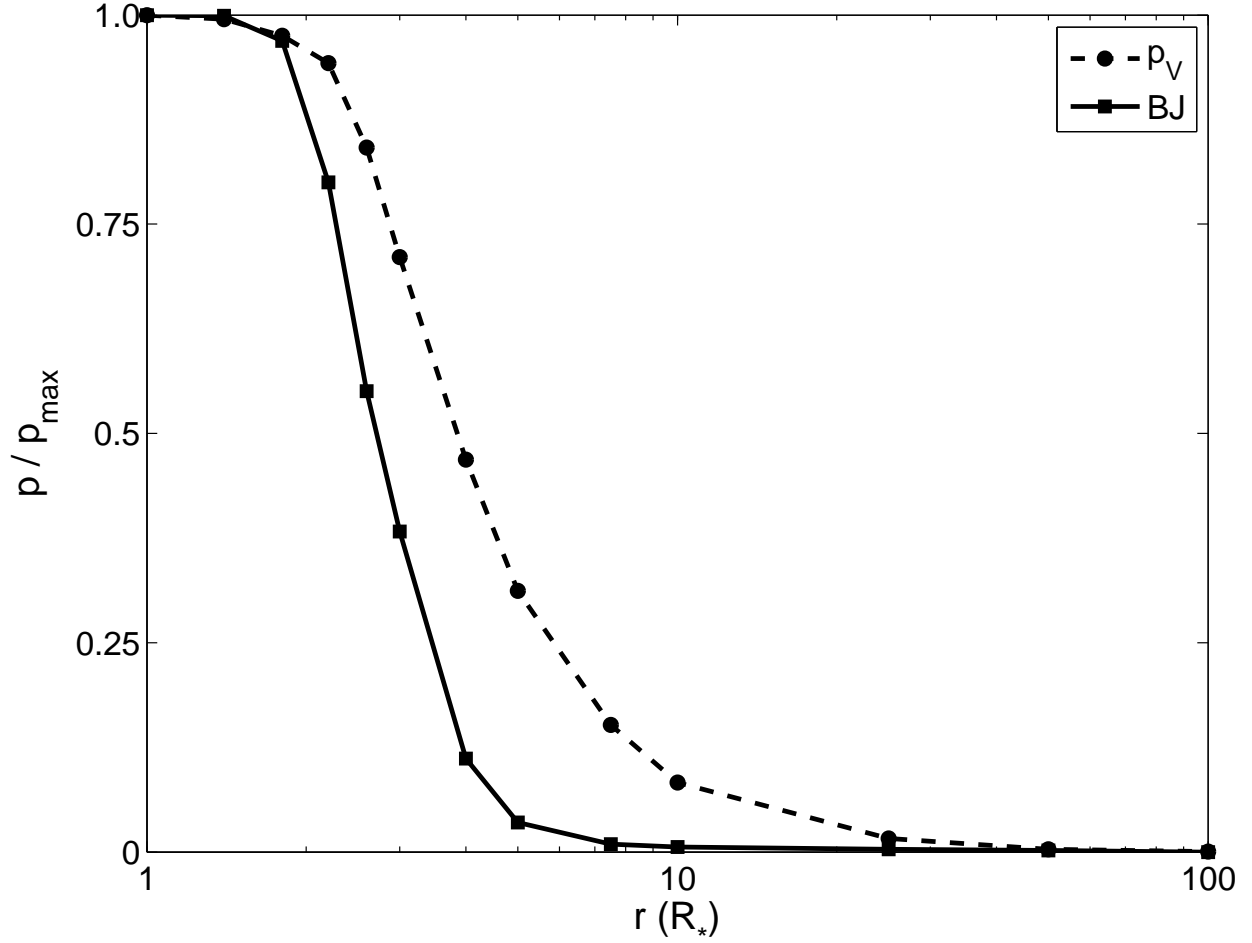
Fig. 8.— Comparison of the change in the polarimetric features for models with circumstellar disks of increasing inner hole radius. The models correspond to a disk with n = 3.5 and with \rho_0 = 1.0 \times 10^{-10} \text{ g cm}^{-3} and inner hole radius ranging from 1.0 R_* to 100.0 R_* . The modeled star is a B2V star viewed at an inclination of i = 75^\circ . The differences between the two quantities in the models reflect that the circumstellar gas is clearing from the inside-out.
