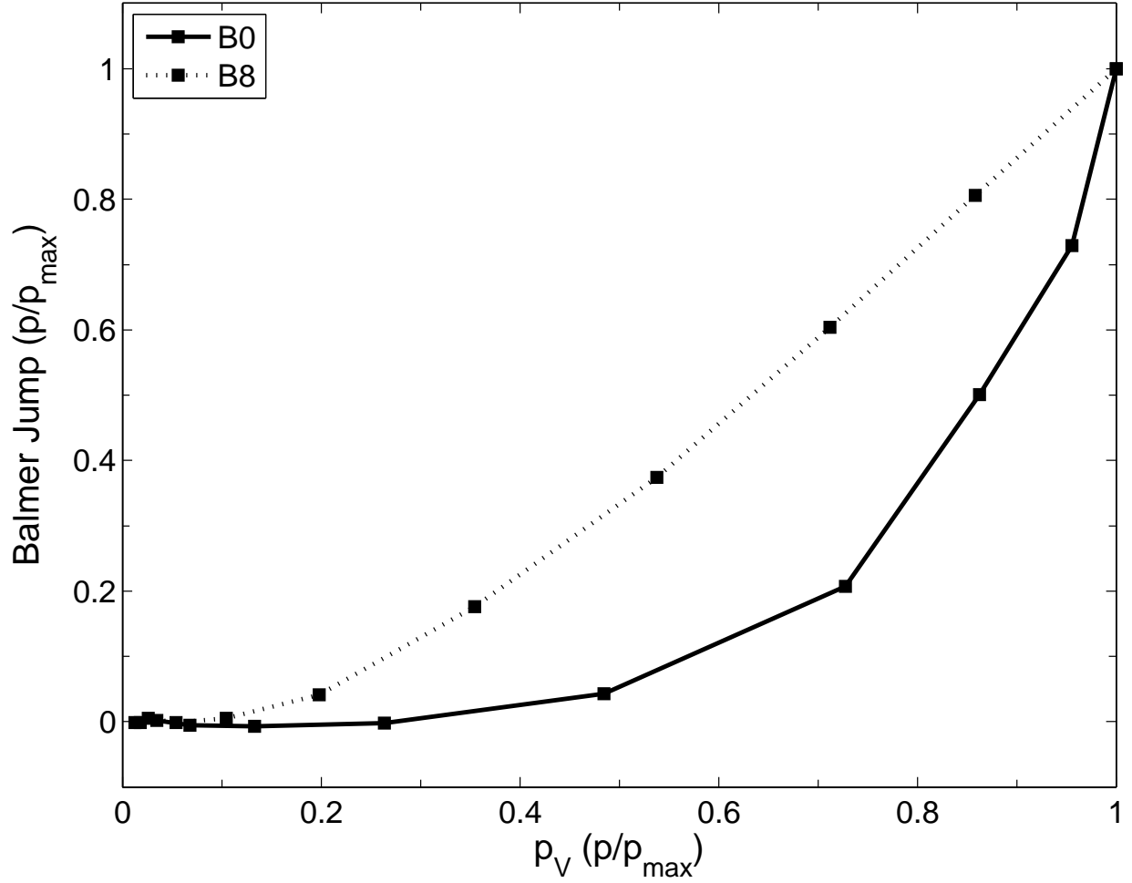
Fig. 11.— BJV curves for disks of increasing mass. The modelled stars are viewed at an inclination of i = 75^\circ and surrounded by a disk with n = 3.5 and with \rho_0 increasing from 3.81 \times 10^{-13} \text{ g cm}^{-3} to 2.0 \times 10^{-10} \text{ g cm}^{-3} .
