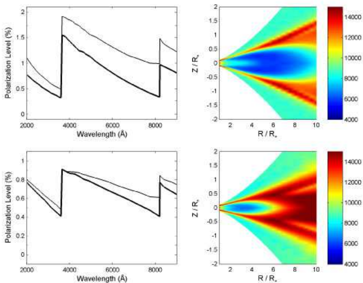
Fig. 4.— Left: Polarization spectra for models using a non-isothermal disk (thin lines) and an isothermal disk (thick lines) viewed at i = 75^\circ . Right: Temperature structure of the non-isothermal disks computed by BEDISK. The models plotted are for B2V stars surrounded by circumstellar disks with n = 3.5 and with \rho_0 = 1.0 \times 10^{-10} \text{ g cm}^{-3} (top) and 2.5 \times 10^{-11} \text{ g cm}^{-3} (bottom).
