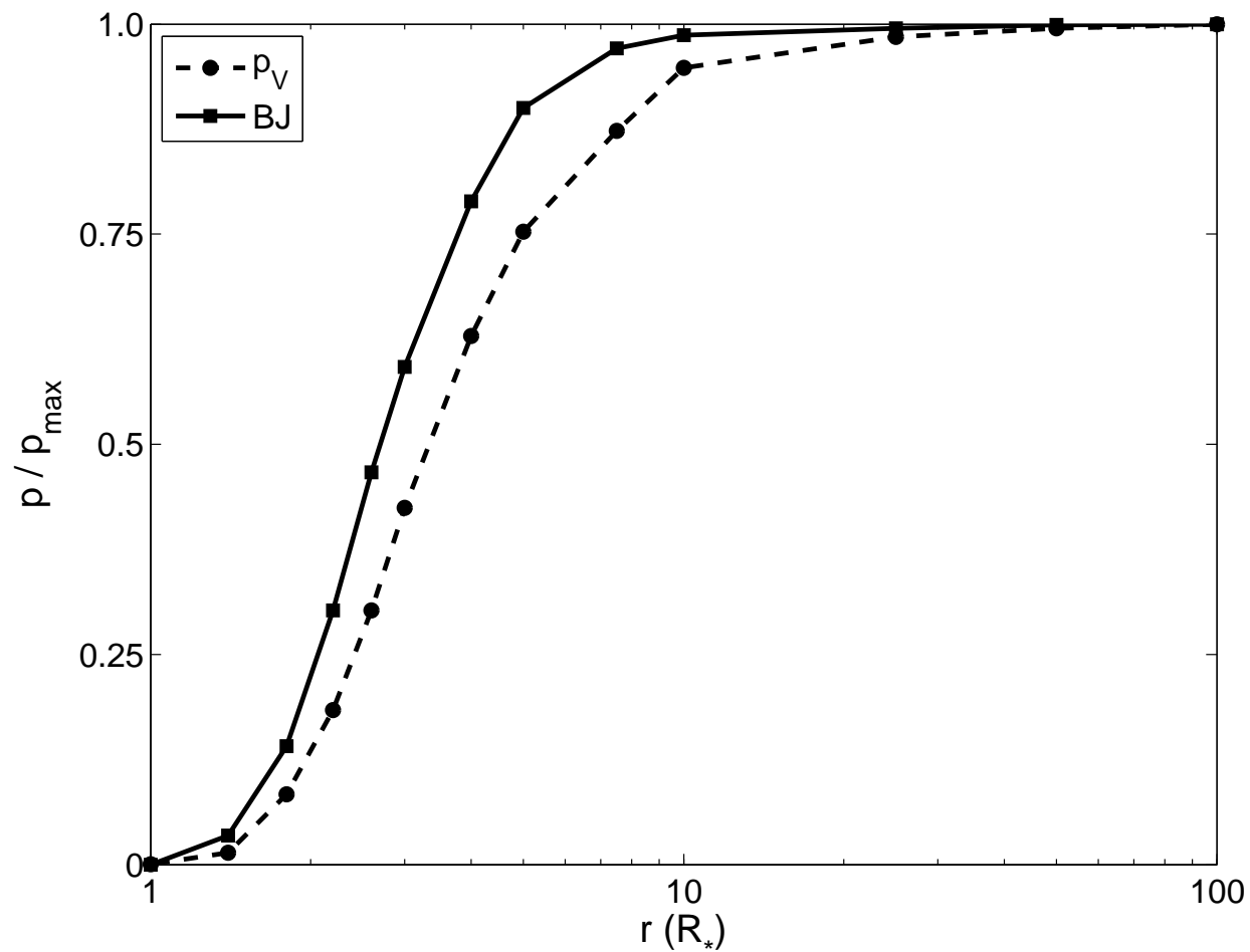
Fig. 6.— Comparison of the growth of polarimetric features for models with circumstellar disks of increasing outer radius. The models correspond to a disk with n = 3.5 and with \rho_0 = 1.0 \times 10^{-10} \text{ g cm}^{-3} and outer radius ranging from 1.0 R_* to 100.0 R_* . The modeled star is a B2V star viewed at an inclination of i = 75^\circ . The differences between the two quantities in the models reflect that gas ejected from the central star is forming an equatorial disk.
