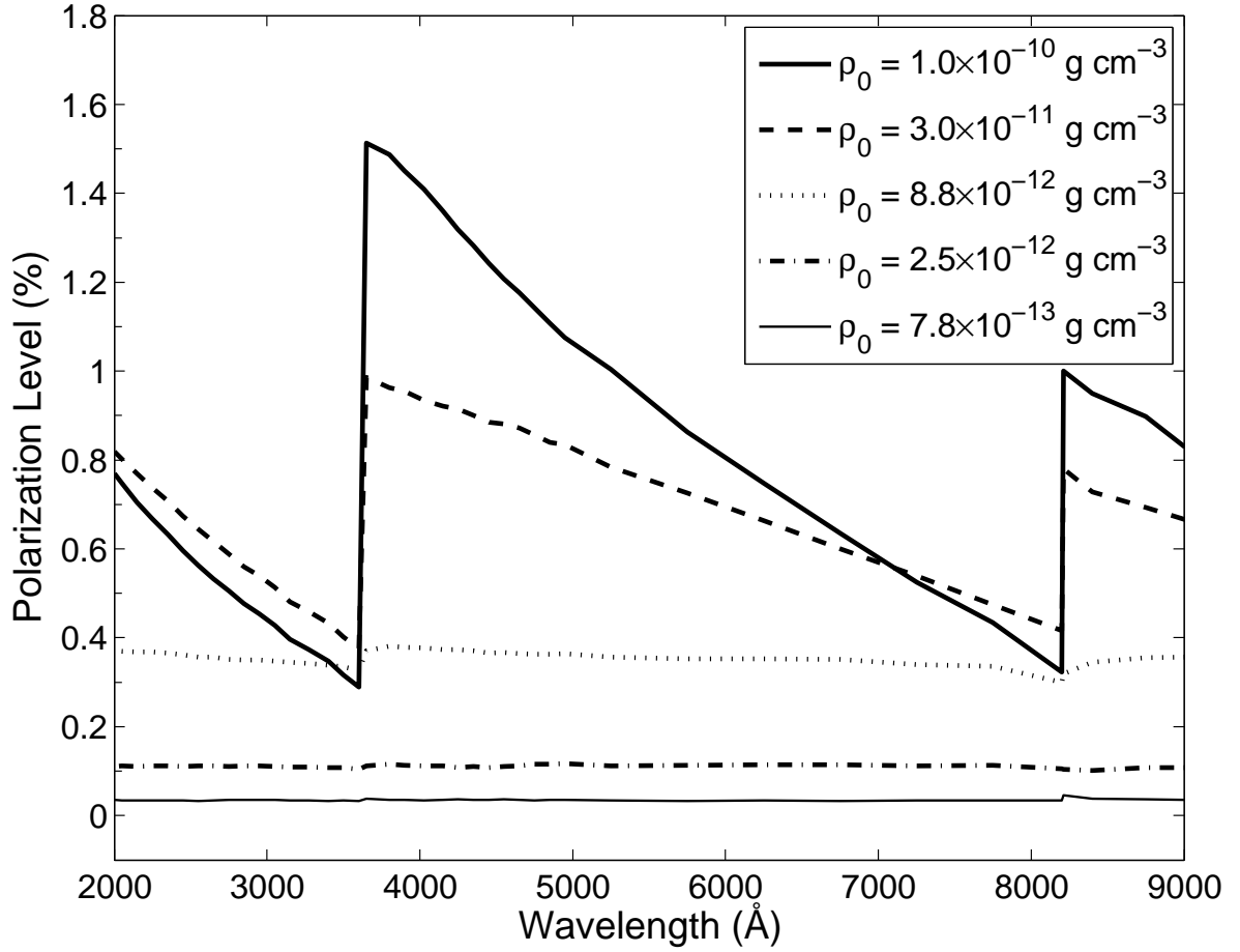
Fig. 1.— Polarization spectra for models with circumstellar disks with varying \rho_0 and with n = 3.5 . The modeled star is a B2V star viewed at an inclination of i = 75^\circ .
