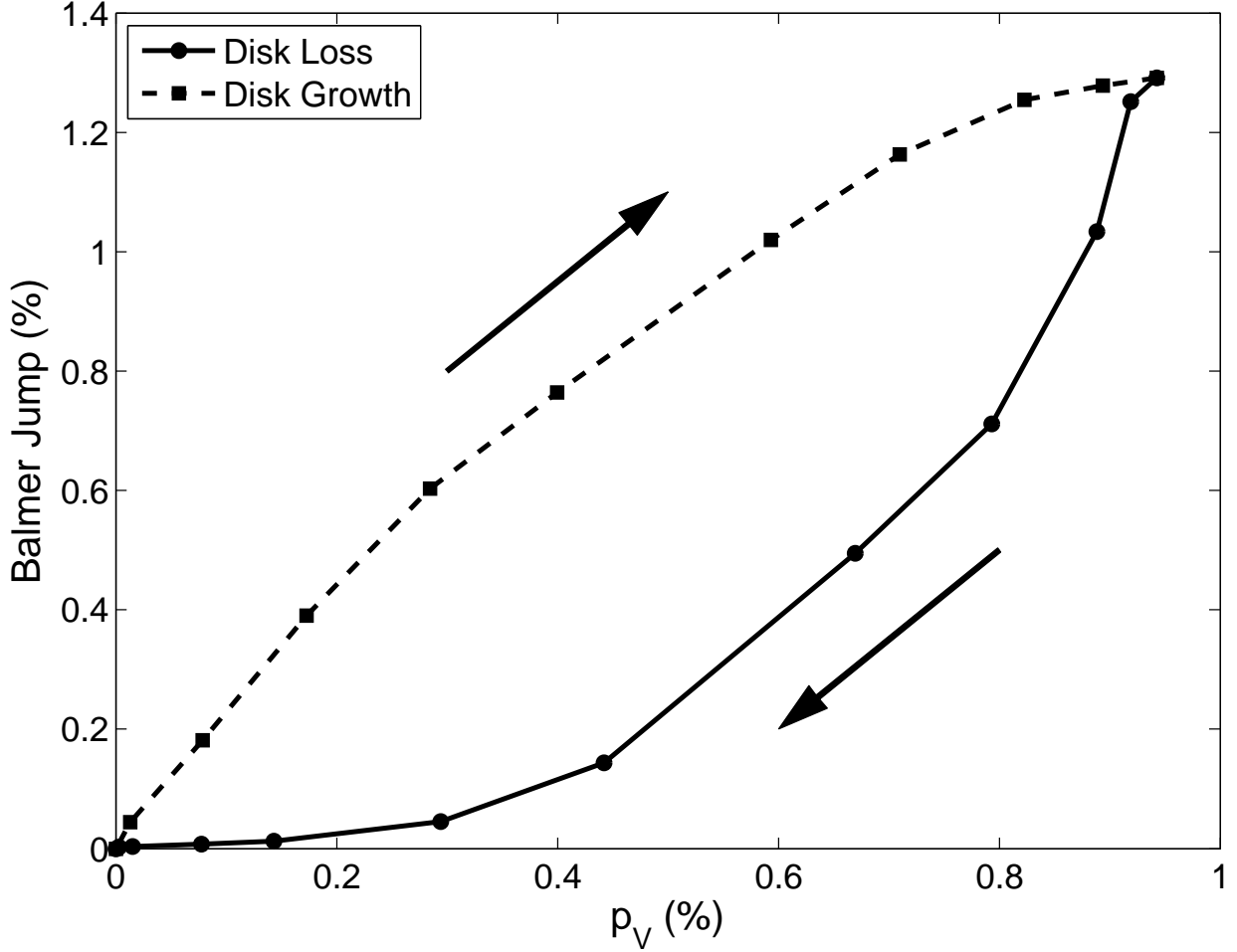
Fig. 9.— BJV loop using the models presented in sections 5.1 and 5.2. The modelled star is a B2V star viewed at an inclination of i = 75^\circ and surrounded by a disk with n = 3.5 and with \rho_0 = 1.0 \times 10^{-10} \text{ g cm}^{-3} . The disk dissipation models correspond to an inner hole of increasing radius ranging from 1.0 R_* to 100.0 R_* . The disk growth models correspond to an increasing outer radius ranging from 1.0 R_* to 100.0 R_* . The evolution of the system, from the moment that mass decrement from the central star begins until the moment where the disk is completely dissipated, traces a clockwise loop in the BJV diagram.
