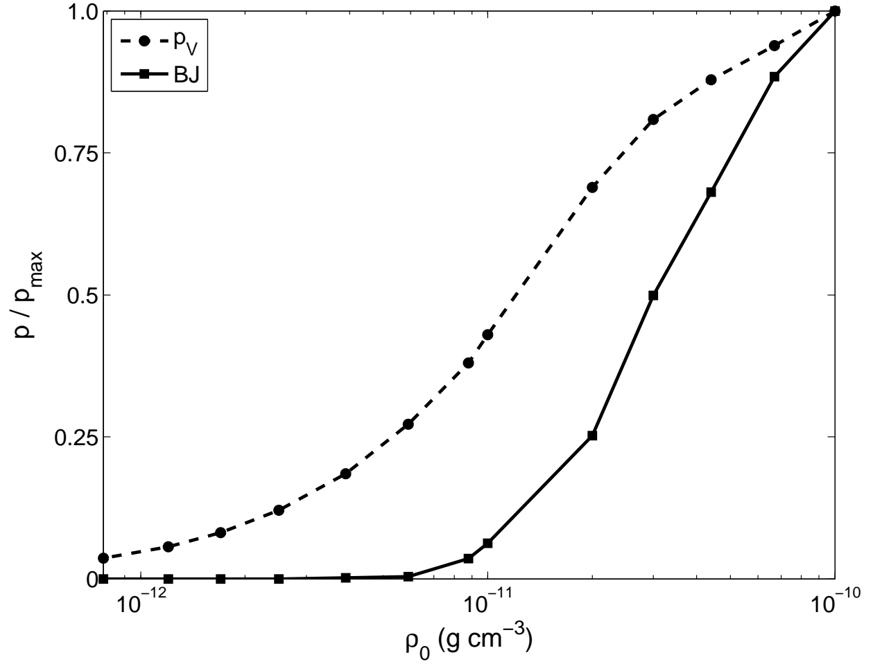
Fig. 2.— Comparison of the growth of polarimetric features (polarization level in V-band p_V and height of Balmer jump BJ ) for models with circumstellar disks with varying \rho_0 and with n = 3.5 . The modeled star is a B2V star viewed at an inclination of i = 75^\circ .
