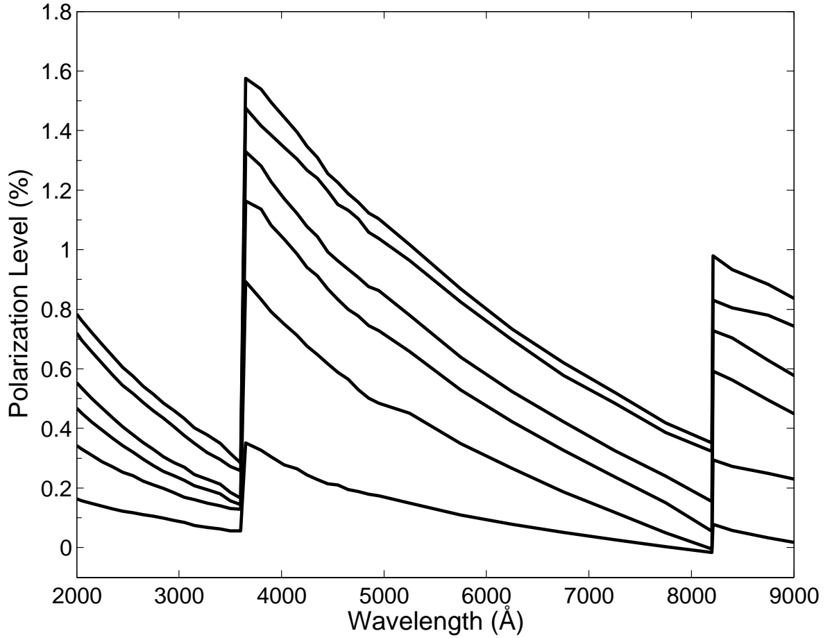
Fig. 5.— Polarization spectra for models with circumstellar disks of increasing outer radius. The models correspond to a disk with n = 3.5 and with \rho_0 = 1.0 \times 10^{-10} \text{ g cm}^{-3} and outer radius, from bottom to top: 2.0 R_* , 3.0 R_* , 4.0 R_* , 5.0 R_* , 10.0 R_* and 100.0 R_* . The modelled star is a B2V star viewed at an inclination of i = 75^\circ .
