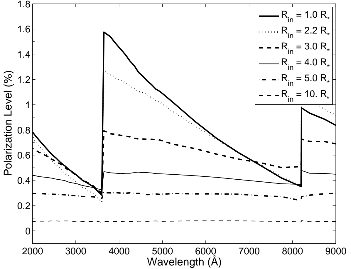
Fig. 7.— Polarization spectra for models with circumstellar disks of increasing inner hole radius. The models correspond to a disk with n and with \rho_0 = 1.0 \times 10^{-10} \text{ g cm}^{-3} . The modeled star is a B2V star viewed at an inclination of i = 75^\circ .
