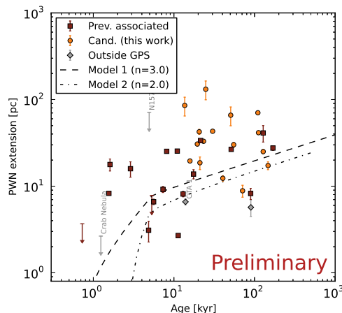
Figure 4: Dependence of measured PWN extensions on characteristic age. The breaks in the models happen at the time when the PWN encounters the SNR reverse shock, which is assumed to happen at 5 kyr (true age, as opposed to characteristic age which is shown in the plot).
