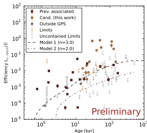
Figure 5: PWN efficiency vs. characteristic age. The yellow limits are likely to enclose the respective PWN, whereas the grey limits are likely to limit only the inner core of it, so the PWN is not fully contained.
