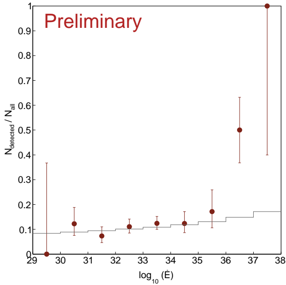
Figure 1: Detection fraction of PMPS pulsars evaluated in bins of \dot{E} . The black histogram at the bottom is the expectation from randomised pulsar populations, see text. The error bar of the highest- \dot{E} bin is large because it is based on only two pulsars.
