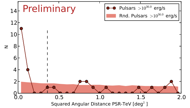
Figure 2: Spatial correlation of high- \dot{E} PMPS pulsars and eligible HGPS source candidates. A clear correlation is seen as a peak at small angular distances, where very few chance coincidences are expected. The dashed line indicates the preliminary criterion to look for preselection candidates, see text.
