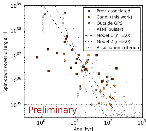
Figure 3: Spin-down power \dot{E} plotted against characteristic age of previously identified PWNe (dark red squares) and preliminary preselection candidates in this work (yellow circles). The grey diamonds are additional PWNe that are not in the HGPS, and the grey dots are other ATNF pulsars for which no TeV counterpart has been detected.
