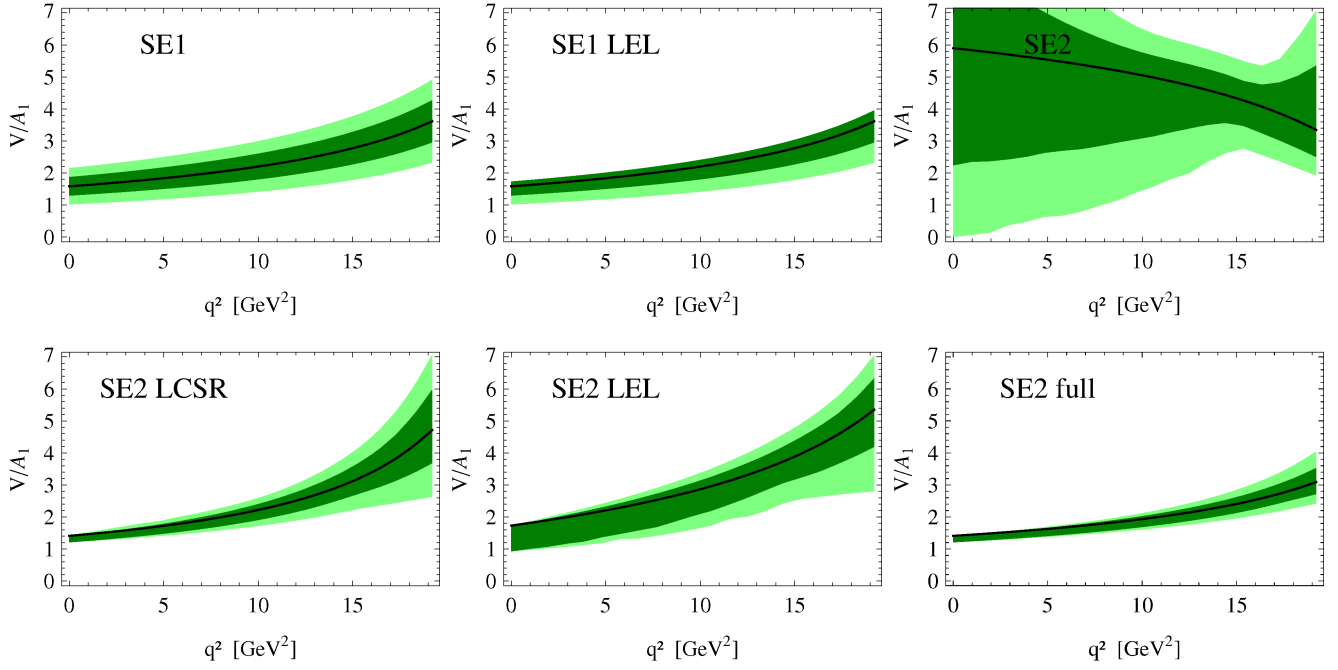
FIG. 8: Fit results as in Fig. 3 for V/A_1 for the full q^2 range.
