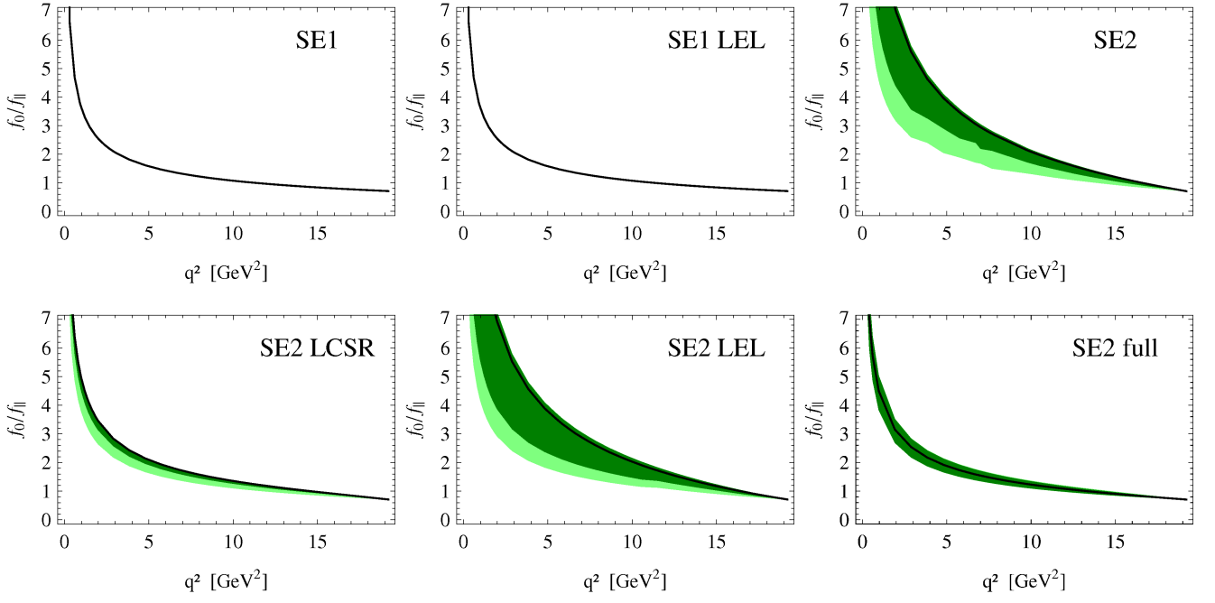
FIG. 6: Fit results as in Fig. 3 for f_0/f_{\parallel} in the full q^2 range. f_0/f_{\parallel} is fixed within the SE1 parametrization.
