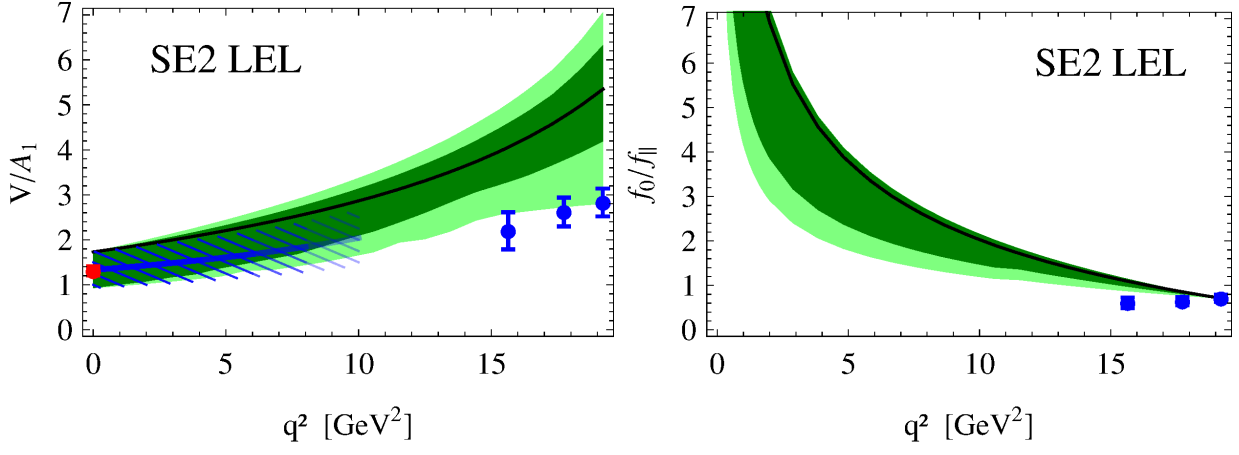
FIG. 10: V/A_1 (left-handed plot) and f_0/f_{||} (right-handed plot) from a fit to data including LEL in SE2 with 68% and 95% C.L. regions shown as dark green and light green bands, respectively. Also shown are lattice results [15] (blue data points), the LCSR ratio Eq. (33) (red point) and the LEL relation Eq. (27) (blue hatched band).
