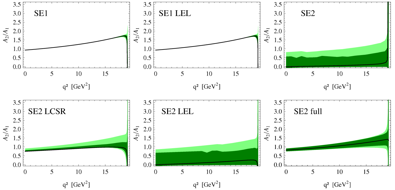
FIG. 9: Fit results as in Fig. 3 for A_2/A_1 in the full q^2 range. A_2/A_1 is fixed within the SE1 parametrization.
