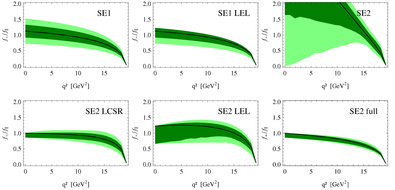
FIG. 7: Fit results as in Fig. 3 for f_{\perp}/f_{\parallel} for the full q^2 range.
