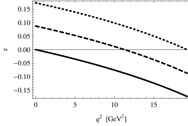
FIG. 2: z(t, t_0) as a function of q^2 in \text{GeV}^2 for t_0 = t_-, t_{opt} and t_0 = 0 , from top to bottom, respectively.
