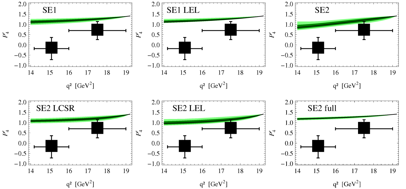
FIG. 5: Current data on P_4' by LHCb (black squares) together with the fit results, see Fig. 3.
