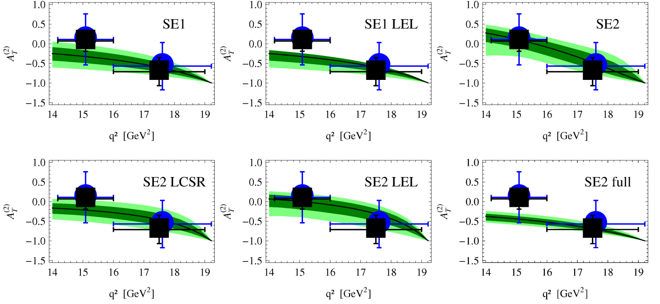
FIG. 4: Current data on A_T^{(2)} by CDF (blue circles) and LHCb (black squares) together with the fit results, see Fig. 3.
