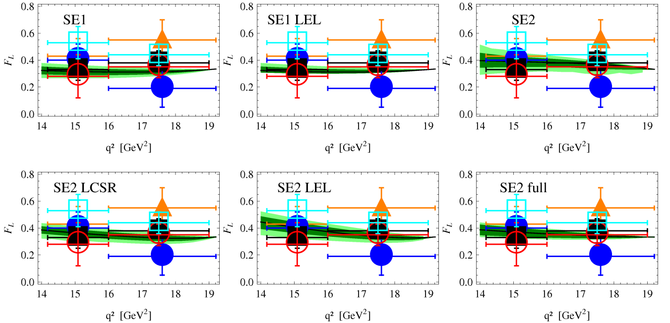
FIG. 3: Current data on F_L by BaBar (orange triangles), CDF (blue circles), LHCb (black squares), ATLAS (blue hollow squares) and CMS (red hollow circles) together with the fit results. 'LEL' and 'LCSR' indicates that the constraints Eq. (45) and Eq. (33), respectively, have been taken into account in the R-fit scheme. 'full' indicates that in addition to the data and LCSR input Eq. (33) the lattice results given in [15] have been taken into account. The SE1 LCSR fit is inconsistent, i.e. , does not work and is not shown, see text for details. The (dark green) light green bands denote the (68%) 95% C.L. regions. The solid black curve corresponds to the best fit result.
