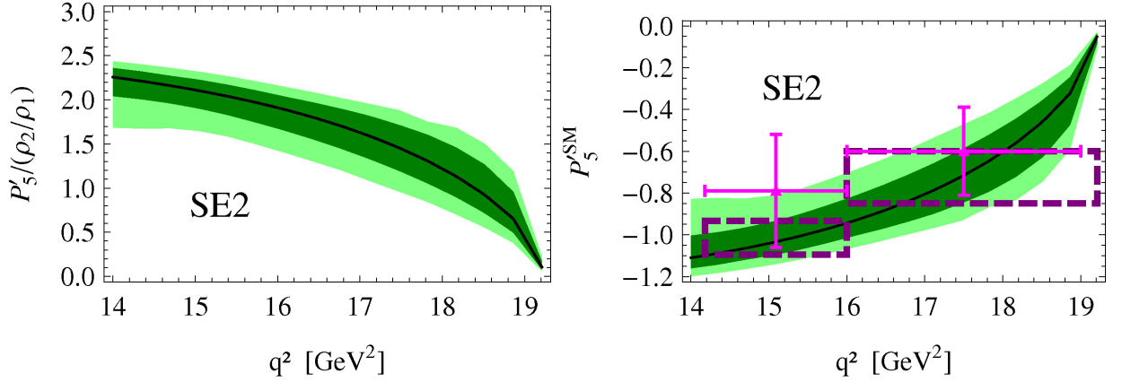
FIG. 13: P'_5/(\rho_2/\rho_1) (left-handed plot) and P_5^{\text{SM}} (right-handed plot) at low recoil from fit to data in SE2. The (68%) 95% C.L. regions are shown in (dark green) light green. The dashed (purple) boxes denote the 1\sigma SM bins. The data points (magenta) correspond to the experimental world average, see Table V.
