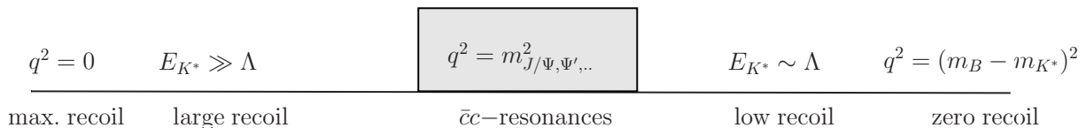
FIG. 1: The regions of interest in the physical spectrum, 4m_\ell^2 \leq q^2 \leq (m_B - m_{K^*})^2 , for B \rightarrow K^* \ell^+ \ell^- decays. The energy of the K^* meson in the B rest frame is given by E_{K^*} = (m_B^2 + m_{K^*}^2 - q^2)/(2m_B) . m_\ell denotes the mass of the leptons. Here we use \Lambda = \Lambda_{\text{QCD}} for the QCD scale. At low recoil the OPE captures the effect of the higher \bar{c}c resonances after sufficiently large q^2 -binning.
