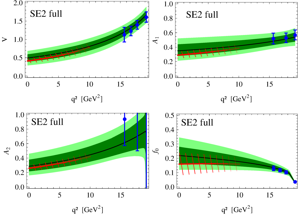
FIG. 11: Form factors in the SE2 full fit scenario, where in addition to the data and the LCSR ratio Eq. (33) the lattice results [15] (blue data points) have been taken into account for V , A_1 and A_2 . The LCSR predictions for form factors [10] (red hatched region) are not included in the fit and are shown for comparison only. The (dark green) light green bands denote the (68%) 95% C.L. regions. The solid black curve corresponds to the best fit result.
