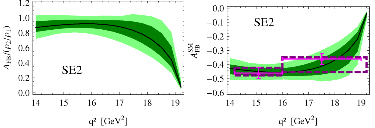
FIG. 12: A_{\text{FB}}/(\rho_2/\rho_1) (left-handed plot) and A_{\text{FB}}^{\text{SM}} (right-handed plot) at low recoil from fit to data in SE2. The (68%) 95% C.L. regions are shown in (dark green) light green. The dashed (purple) boxes denote the 1\sigma SM bins. The data points (magenta) correspond to the experimental world average, see Table IV.
