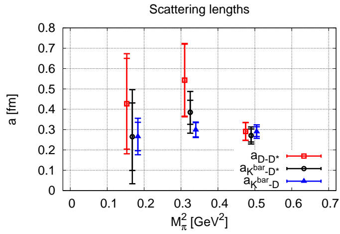
Figure 4: (color online) Pion mass dependences of scattering lengths in the I = 0 \bar{K}-D , \bar{K}-D^* and D-D^* channels. Inner vertical error bars represent statistical errors. Both statistical and systematic errors are included in total error bars.
