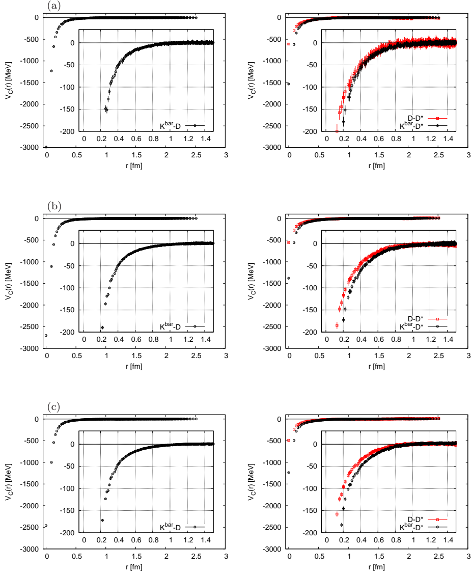
Figure 2: (color online) Left three panels for the S-wave central potentials in the \bar{K}-D channel with (J^P, I) = (0^+, 0) . Right three panels for the S-wave central potentials in the D-D^* (square) and \bar{K}-D^* (circle) channels with (J^P, I) = (1^+, 0) . (a), (b) and (c) are obtained at m_\pi \simeq 410 MeV, m_\pi \simeq 570 MeV and m_\pi \simeq 700 MeV, respectively.
