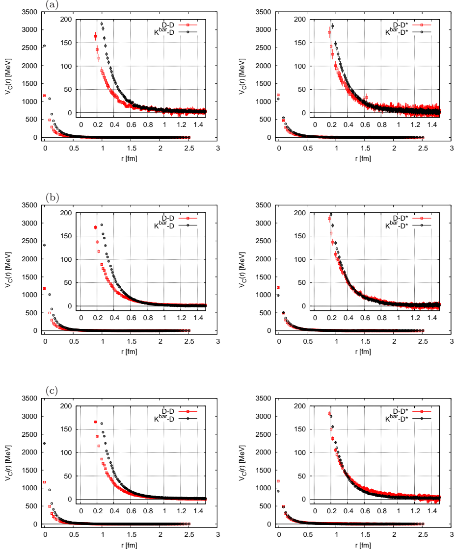
Figure 1: (color online) Left three panels for the S-wave central potentials in the D - D (square) and \bar{K} - D (circle) channels with (J^P, I) = (0^+, 1) . Right three panels for the S-wave central potentials in the D - D^* (square) and \bar{K} - D^* (circle) channels with (J^P, I) = (1^+, 1) . (a), (b) and (c) are obtained at m_\pi \simeq 410 MeV, m_\pi \simeq 570 MeV and m_\pi \simeq 700 MeV, respectively.
