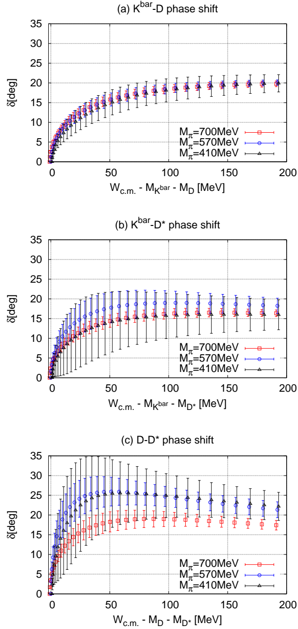
Figure 3: (color online) S-wave I = 0 scattering phase shifts in the (a) \bar{K}-D , (b) \bar{K}-D^* and (c) D-D^* channels. Vertical error bars represent both statistical and systematic errors.
