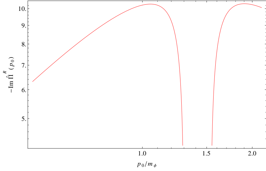
Figure 7: The imaginary part of the retarded \chi -self-energy \text{Im}\hat{\Pi}_{\chi\mathcal{P}}^R(p_0) \equiv \text{Im}\Pi_{\chi\mathcal{P}}^R(p_0)/g^2 for g = m_\chi = m_\phi/6 , T = 333m_\phi and |\mathbf{p}| = m_\phi as a function of p_0 .
