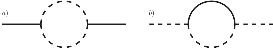
Figure 1: Diagrams contributing to the self-energies for \phi , a), and \chi , b), at on-loop order. Solid lines represent \phi -propagators, dashed lines \chi -propagators.
