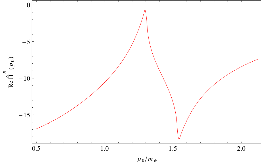
Figure 6: The real part of the retarded \chi -self-energy \text{Re}\hat{\Pi}_{\chi p}^R(p_0) \equiv \text{Re}\Pi_{\chi p}^R(p_0)/g^2 for g = m_\chi = m_\phi/6 , T = 333m_\phi and |\mathbf{p}| = m_\phi as a function of p_0 .
