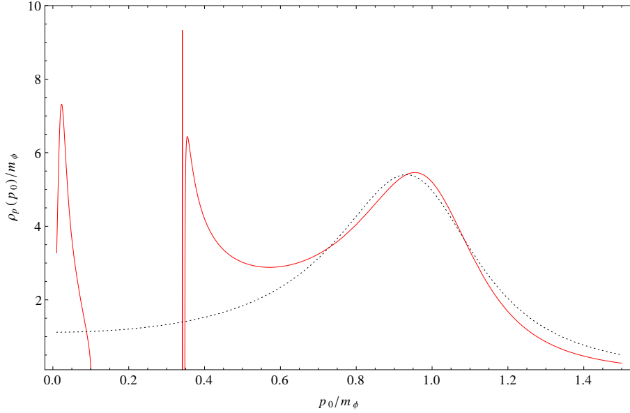
Figure 5: Solid red line: The spectral density \rho_{\phi\mathbf{p}}(p_0) from (5) with g = m_\chi = m_\phi/6 , T = 333m_\phi and |\mathbf{p}| = m_\phi/10 as a function of p_0 . The isolated feature near p_0 \simeq 0.34m_\phi represents a \delta -function, which we interpret as a novel scalar plasmon of purely collective origin, the luon . Another interesting feature is the continuous contribution for p^2 < 0 , which disappears in the limit T \rightarrow 0 . Dotted black line: The Breit-Wigner approximation (8) in the vicinity of the screened particle pole.
