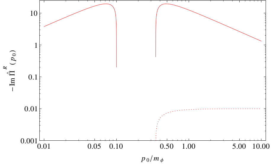
Figure 3: The imaginary part of the retarded \phi -self-energy \text{Im}\hat{\Pi}_{\phi p}^R(p_0) \equiv \text{Im}\Pi_{\phi p}^R(p_0)/g^2 for m_\chi = m_\phi/6 , T = 333m_\phi and |\mathbf{p}| = m_\phi/10 as a function of p_0 . The dotted line is the T = 0 contribution.
