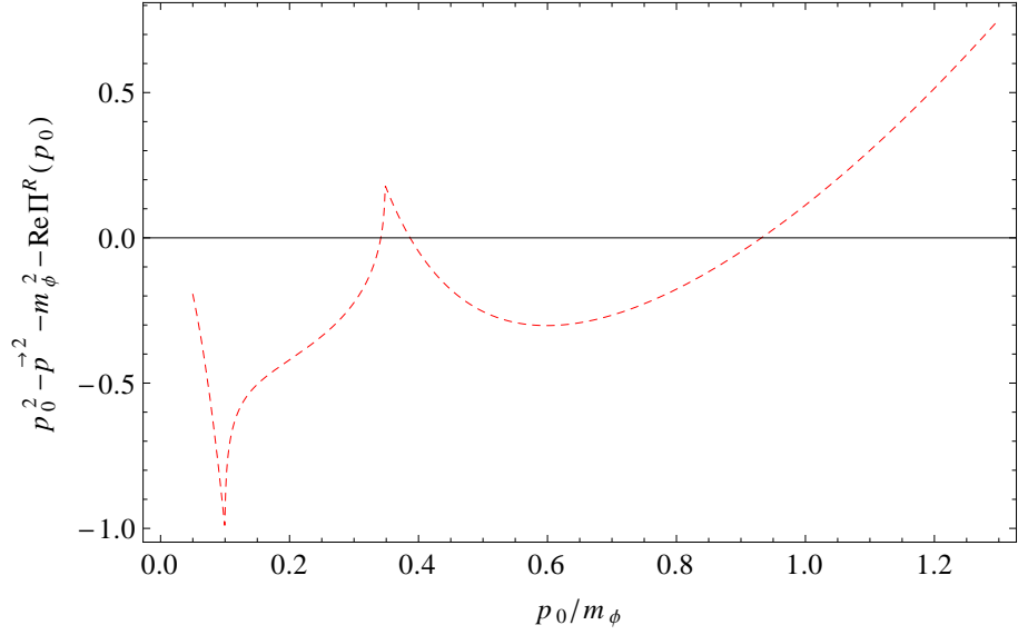
Figure 4: The left hand side of (16) for g = m_\chi = m_\phi/6 , T = 333m_\phi and |\mathbf{p}| = m_\phi/10 as a function of p_0 .
