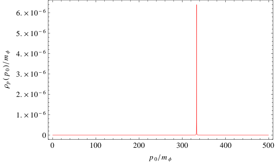
Figure 9: The spectral density \rho_{\chi P}(p_0) for \chi with g = m_\chi = m_\phi/6 , T = 333m_\phi and |\mathbf{p}| = T as a function of p_0 .
