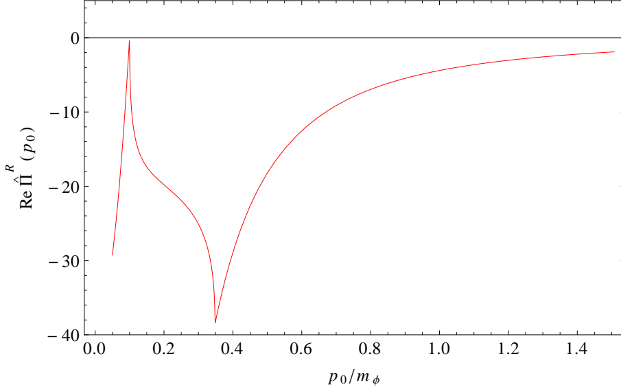
Figure 2: The real part of the retarded \phi -self-energy \text{Re}\hat{\Pi}_{\phi\mathbf{p}}^R(p_0) \equiv \text{Re}\Pi_{\phi\mathbf{p}}^R(p_0)/g^2 for m_\chi = m_\phi/6 , T = 333m_\phi and |\mathbf{p}| = m_\phi/10 as a function of p_0 . The function is positive for p_0 \gg m_\phi .
