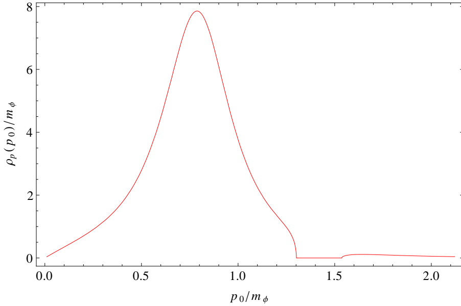
Figure 8: The spectral density \rho_{\mathcal{P}}(p_0) with g = m_\chi = m_\phi/6 , T = 333m_\phi and |\mathbf{p}| = m_\phi as a function of p_0 .
