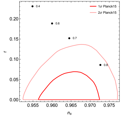
Figure 1: We compare the theoretical predictions in the r - n_s plane for different values of \delta with Planck '15 results for TT, TE, EE, +lowP and assuming \Lambda CDM + r [51]. We used the complete expression for the quantum corrected potential in (1) and further assumed \mu_0 = 10^{-3} M_{\text{P}}
