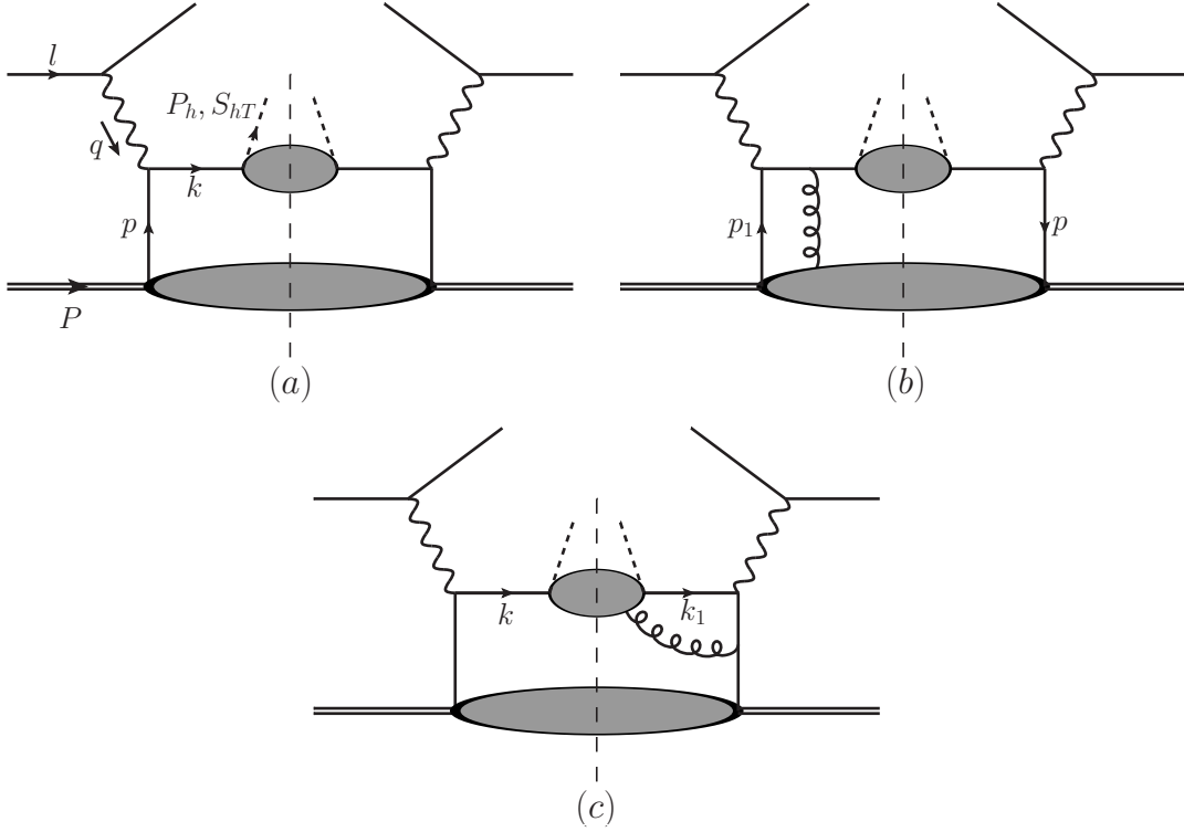
Figure 1: Graphs showing the relevant channels for \ell p \rightarrow \Lambda^\uparrow X within collinear twist-3 factorization. The diagram in (a) involves qq correlators, while the ones in (b), (c) (and their Hermitian conjugates) deal with qqg correlators.
