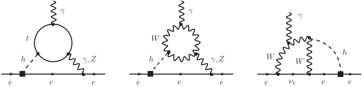
Figure 4: Sample two-loop Feynman diagrams inducing an EDM for the electron through a CP-violation Higgs coupling to the electron (here denoted by the black square).
