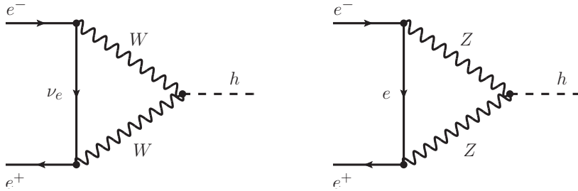
Figure 5: Sample one-loop Feynman diagrams which naively look like they might give a SM s -channel Higgs production cross section that is not suppressed by the small electron Yukawa. As shown in the text, chiral symmetry implies that the amplitude for this process is suppressed by the electron mass for on-shell external fermions.
