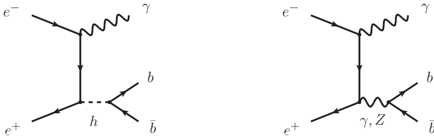
Figure 2: Resonant Higgs boson production at LEP II via radiative return to the Higgs pole (left diagram). The Higgs is assumed to decay into a b\bar{b} final state. The main background is given by off-shell photons or Z bosons decaying into a b\bar{b} pair (right diagram).
