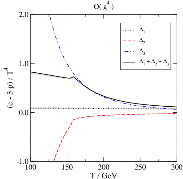
Figure 3: The trace “anomaly” from eq. (7.1). The grey band reflects variations of the renormalization scale in the range \bar{\mu} = (0.5\dots 2.0)\pi T . Contributions of \mathcal{O}(\nu^4/T^4) are seen to cancel at low temperatures.
