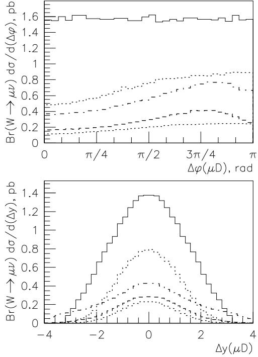
Figure 1: Kinematic correlations between muons and D -mesons in same-sign events ( \mu^\pm D^\pm ) at ATLAS conditions: distributions in the azimuthal angle difference \Delta\phi (upper panel) and rapidity difference \Delta y (lower panel). The different contributions are represented by: solid curve, double parton scattering; upper dotted curve, gg \rightarrow t\bar{t} ; lower dotted curve, q\bar{q} \rightarrow t\bar{t} ; dashed curve, u\bar{d} \rightarrow W c\bar{c} and d\bar{u} \rightarrow W c\bar{c} ; dash-dotted curve, gu \rightarrow W d c\bar{c} and gd \rightarrow W u c\bar{c} .
