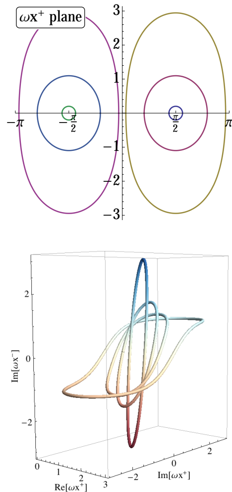
FIG. 3. Upper panel: The two instantons (18) in the sinusoidal field (17), for r = 1/10, 1/2, 99/100 (expanding outward). The instantons circulate the electric field maxima at \omega x^+ = \pm\pi/2 . Lower panel: A projection of the instantons in x^+-x^- space, circulating \omega x^+ = \pi/2 and x^- = 0 , for \omega = \mathcal{E} and various r .
