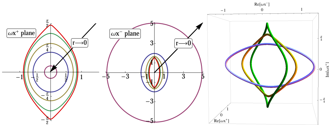
FIG. 2. Left : The x^+ instantons in the Sauter pulse for r = 1/5, 3/5, 4/5, 19/20, 999/1000 . As r \rightarrow 0 the instantons contract to the origin, while as r \rightarrow 1 they are reflected from the poles of the electric field at \omega x^+ = \pm\pi/2 [23]. Middle : The x^- instantons for the same values of r and \omega = \mathcal{E} , which expand as the x^+ instantons contract. Right : A projection of the instantons in x^+-x^- space for r = 3/5, 4/5, 19/20 (blue, yellow, green).
