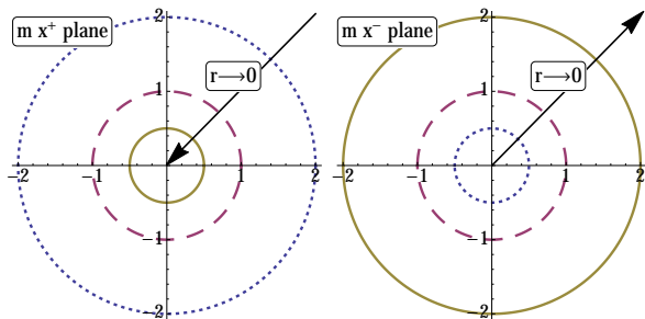
FIG. 1. The complex instantons in a constant electric field for r = 2, 1, 1/2 (dotted, dashed, solid) and \mathcal{E} = m . As r \rightarrow 0 the x^+ instanton shrinks to a point, while the x^- instanton expands.
