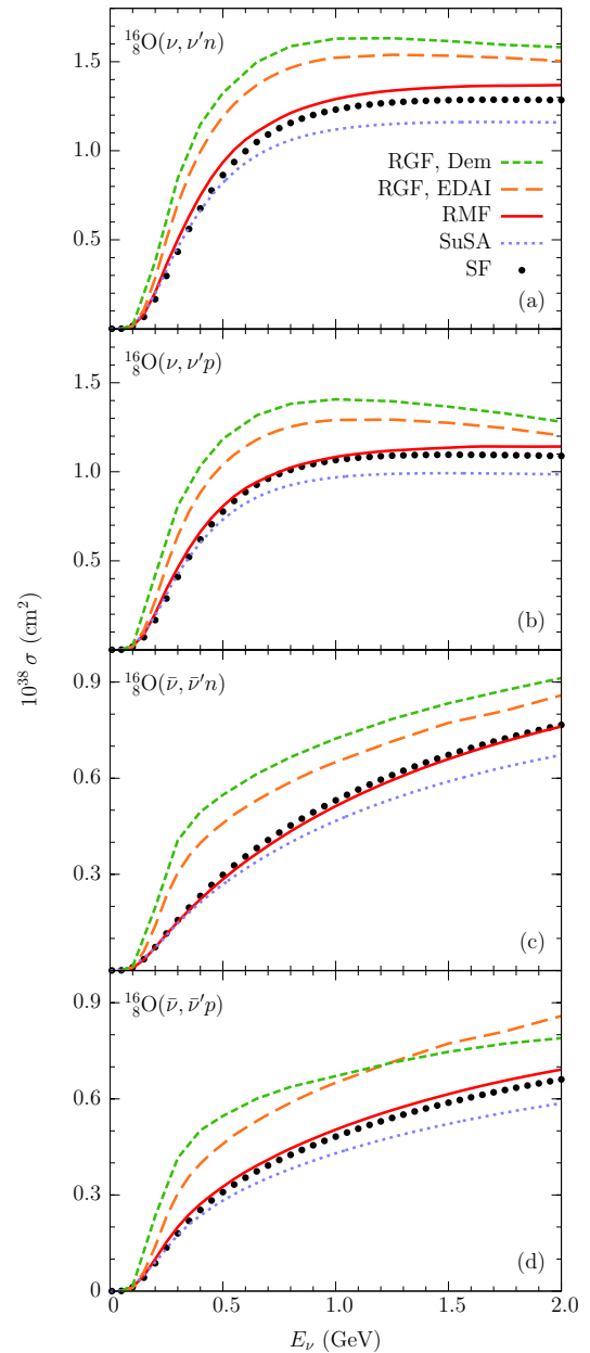
FIG. 2. (Color online) Same as in Fig. 1 but for the SuSA model (dotted lines), the RMF approach (solid lines), and the RGF calculations with the EDAI (long-dashed lines) and “democratic” (short-dashed lines) potentials. For comparison, we also include the SF results displayed in Fig. 1, represented by filled circles.
