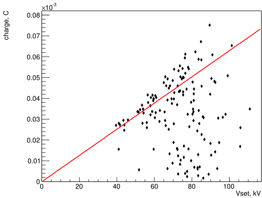
Figure 11. Correlations between integrated charge and breakdown voltage V_{set} for the selected events with distinguishable slow streamer phase (top) and for all events with recorded current characteristics (bottom). The red line represents the charge stored in the gap capacitance using the tuned value of the latter.
