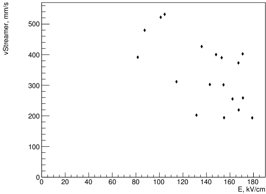
Figure 15. Correlations between minimum streamer velocity v_{Streamer} and maximum breakdown field E for the selected events with a distinguishable slow streamer phase.
