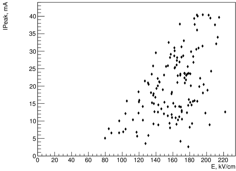
Figure 12. Correlations between peak current I_{Peak} and maximum breakdown field E for all events with recorded current characteristics.
