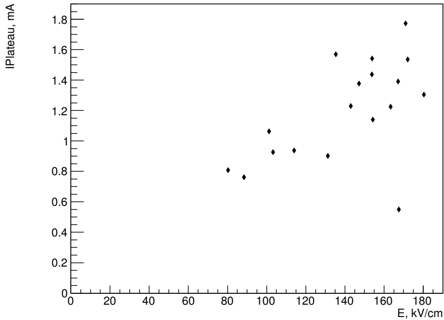
Figure 13. Correlations between plateau current I_{Plateau} and maximum breakdown field E for the selected events.
