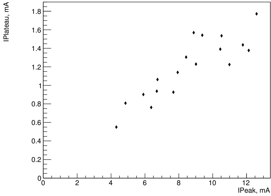
Figure 14. Correlations between plateau current I_{Plateau} and peak current I_{Peak} for the selected events.
