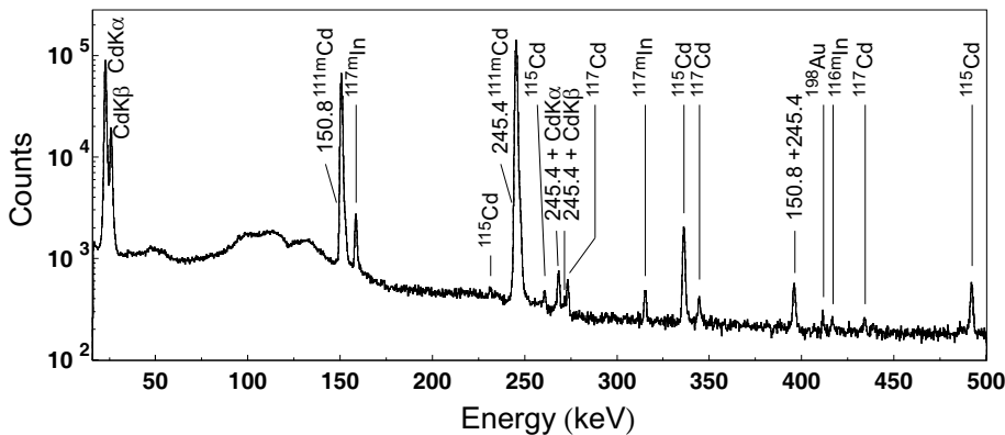
FIG. 2: Portion of the x- and \gamma -ray energy spectrum measured for 15 min with source S2. Room background has been subtracted. Peaks are labeled by their \beta -decay parent; the \gamma -ray peaks associated with ^{111m}\text{Cd} decay also have their energies in keV marked.
