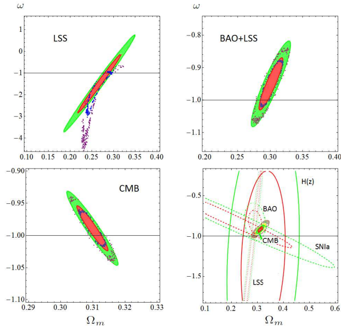
FIG. 6.— Upper-left plot : two-dimensional \Omega_m - \omega contours at 1\sigma and 2\sigma c.l. for the \Lambda CDM, obtained with only the LSS data set. The dotted contours in blue and purple are the exact ones, whilst the red and green ellipses have been obtained using the Fisher’s approximation. Upper-right plot : Same, but for the combination BAO+LSS. Lower-left plot : As in the upper plots, but for the CMB data. Lower-right plot : The Fisher’s generated contours at 1\sigma and 2\sigma c.l. for all the data sets: SN Ia (dotted lines), H(z) (solid lines), BAO (dot-dashed lines), LSS (dotted, very thin lines) and CMB (solid lines, tightly packed in a very small, segment-shaped, region at such scale of the plot). The exact, final, combined contours (from 1\sigma up to 5\sigma ) can be glimpsed in the small colored area around the center. See the text for further explanations and Fig. 3 for a detailed view.
