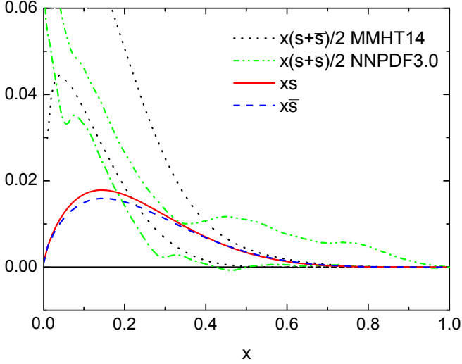
Figure 3: Comparison between the strange x s (solid red curve) and antistrange x \bar{s} (dashed blue curve) PDFs from kaon loops, for the cutoff parameters ( \mu_1 = 545 MeV and \mu_2 = 600 MeV) that give the maximum total s + \bar{s} , with the upper and lower limits of the error bands for x(s + \bar{s})/2 at Q^2 = 1 GeV 2 from the MMHT14 [51] (black dotted) and NNPDF3.0 [52] (green dot-dashed) global fits.
