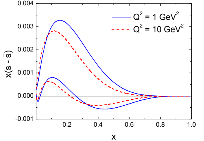
Figure 4: Strange quark asymmetry x(s - \bar{s}) at Q^2 = 1 GeV 2 (solid blue curves) and evolved to Q^2 = 10 GeV 2 (dashed red curves). The upper (lower) curves correspond to the maximum (minimum) value for S^- = 1.12 \times 10^{-3} ( -0.07 \times 10^{-3} ), for cutoff parameters \mu_1 = 526 MeV, \mu_2 = 894 MeV ( \mu_1 = 545 MeV, \mu_2 = m_K ).
