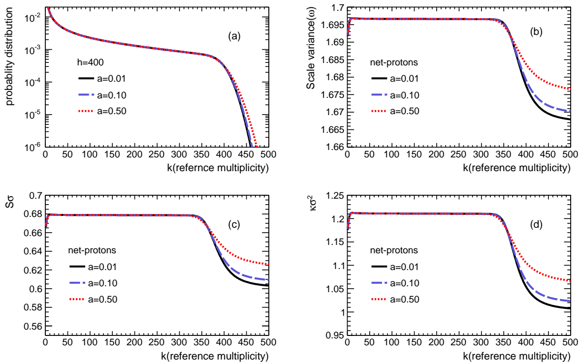
FIG. 2. (Color online) (a) Distributions of reference multiplicity and cumulant products (b) \omega = c_2/c_1 , (c) S\sigma = c_3/c_2 , (d) \kappa\sigma^2 = c_4/c_2 of net proton distributions with various strength of Gaussian-type external volume fluctuations a = 0.01 (black-solid lines), a = 0.10 (blue-dashed lines) and a = 0.50 (red-dotted lines).
