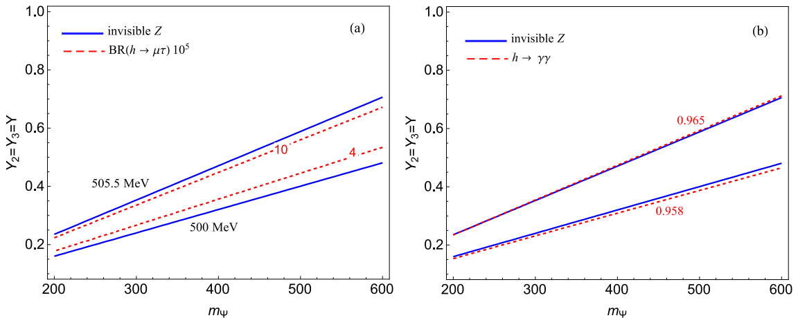
FIG. 1: Contours as a function of Y and m_\Psi : (a) for \Gamma(Z \rightarrow \nu_i\nu_j) and BR(h \rightarrow \mu\tau) and (b) for signal strength \mu_{\gamma\gamma} , where the numbers on the plot (a) for BR(h \rightarrow \mu\tau) are in units of 10^{-5} .
