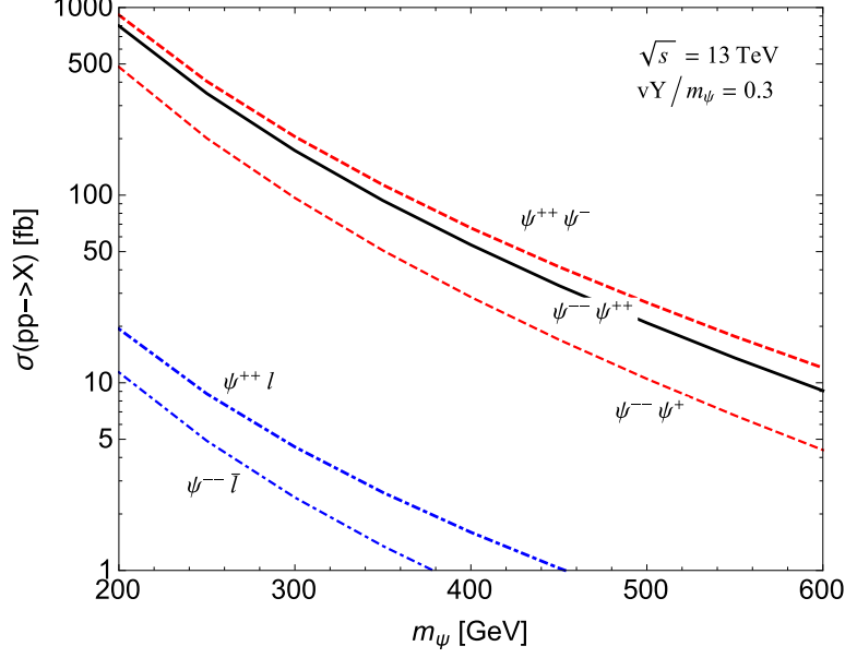
FIG. 3: Doubly charged lepton production cross section ( in units of fb) as a function of m_\Psi in pp collisions at \sqrt{s} = 13 TeV, where X in the y-axis denotes the possible channel.
