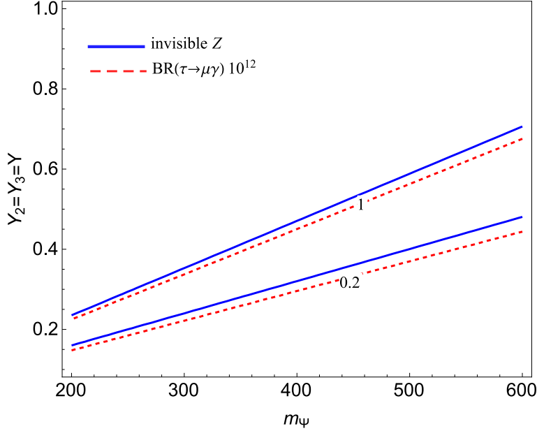
FIG. 2: Contours for BR(\tau \rightarrow \mu\gamma) (dashed) as a function of Y and m_\Psi , where the constraint from \Gamma_{\text{inv}}^Z (solid) is included.
